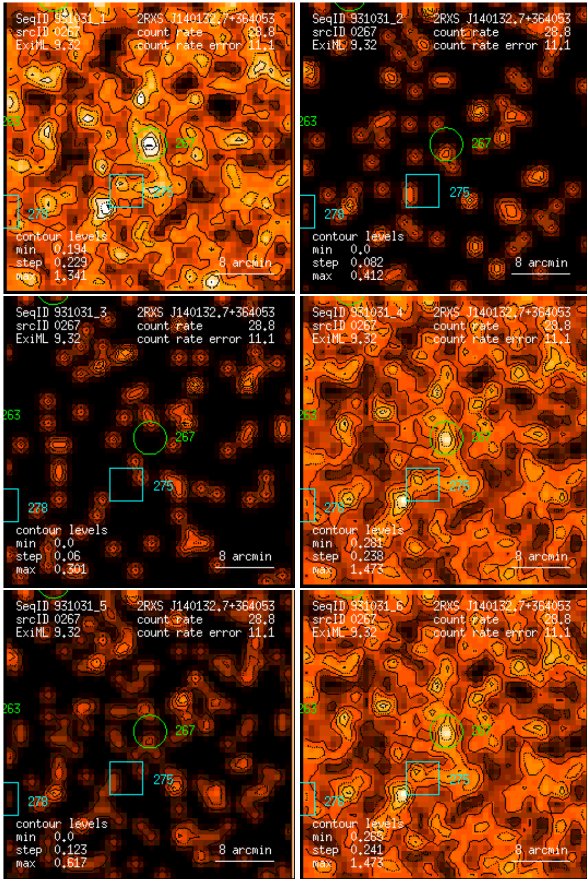
Figure 267: RASS 931031: detection 0267: band rate images, Gaussian filter: (1) PSPC channels 11 – 41, (2) 52 – 90, (3) 91 – 201, (4) 11 – 235, (5) 52 – 201, (6) 11 – 201. Broad band rates in counts/ks. Band rate contour levels in counts/ks/arcmin 2 .
