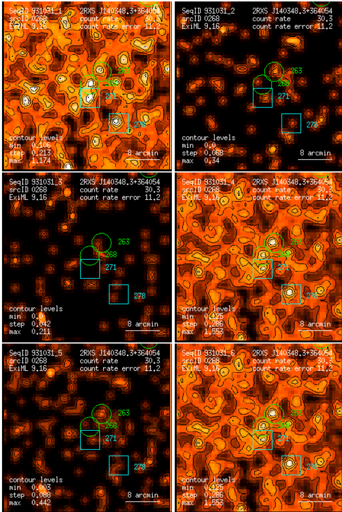
Figure 268: RASS 931031: detection 0268: band rate images, Gaussian filter: (1) PSPC channels 11 – 41, (2) 52 – 90, (3) 91 – 201, (4) 11 – 235, (5) 52 – 201, (6) 11 – 201. Broad band rates in counts/ks. Band rate contour levels in counts/ks/arcmin 2 .
