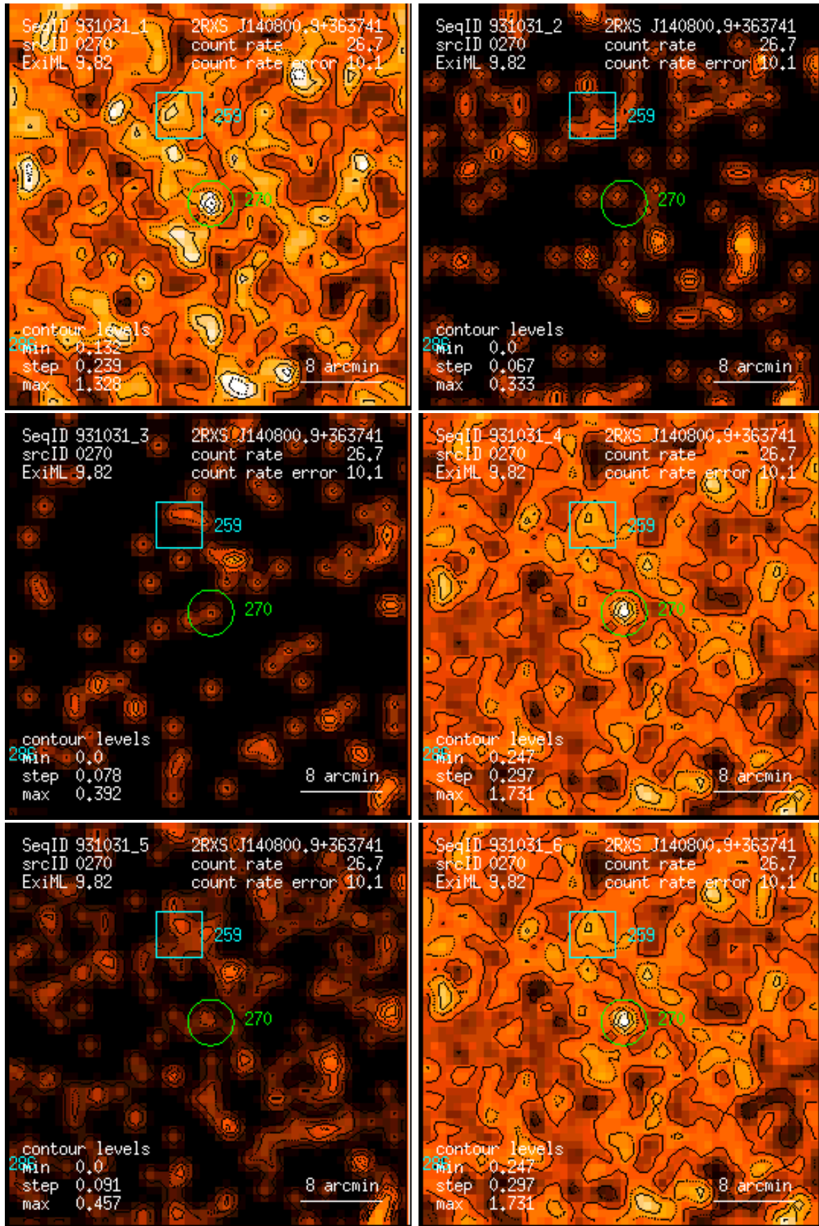
Figure 270: RASS 931031: detection 0270: band rate images, Gaussian filter: (1) PSPC channels 11 – 41, (2) 52 – 90, (3) 91 – 201, (4) 11 – 235, (5) 52 – 201, (6) 11 – 201. Broad band rates in counts/ks. Band rate contour levels in counts/ks/arcmin 2 .
