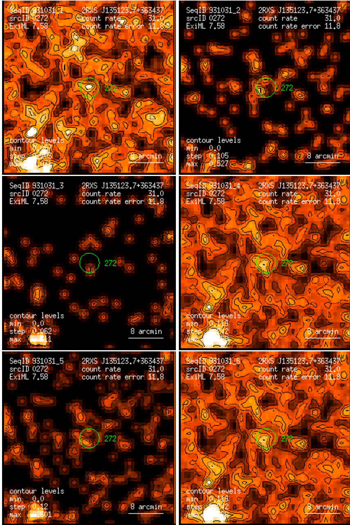
Figure 272: RASS 931031: detection 0272: band rate images, Gaussian filter: (1) PSPC channels 11 – 41, (2) 52 – 90, (3) 91 – 201, (4) 11 – 235, (5) 52 – 201, (6) 11 – 201. Broad band rates in counts/ks. Band rate contour levels in counts/ks/arcmin 2 .
