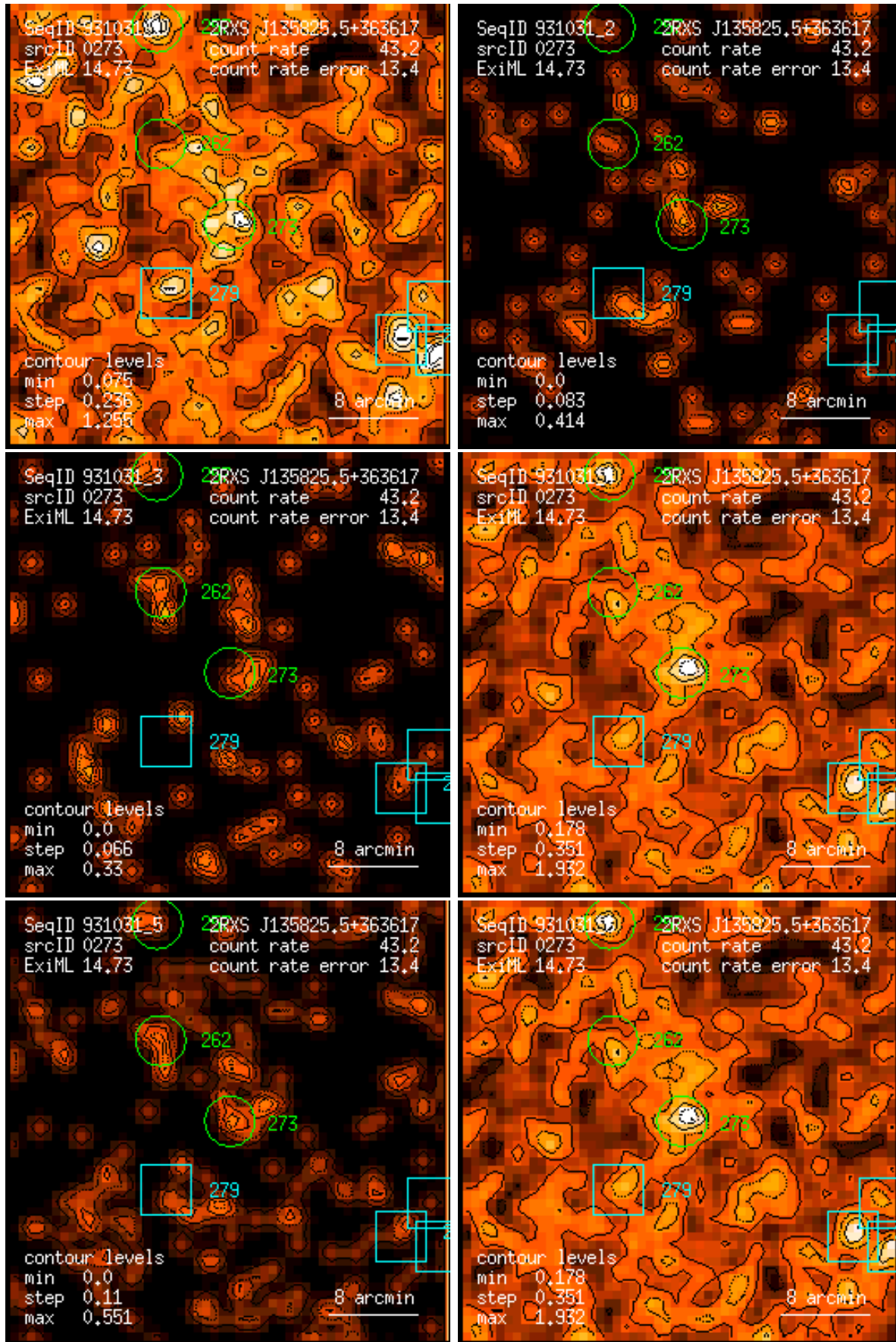
Figure 273: RASS 931031: detection 0273: band rate images, Gaussian filter: (1) PSPC channels 11 – 41, (2) 52 – 90, (3) 91 – 201, (4) 11 – 235, (5) 52 – 201, (6) 11 – 201. Broad band rates in counts/ks. Band rate contour levels in counts/ks/arcmin 2 .
