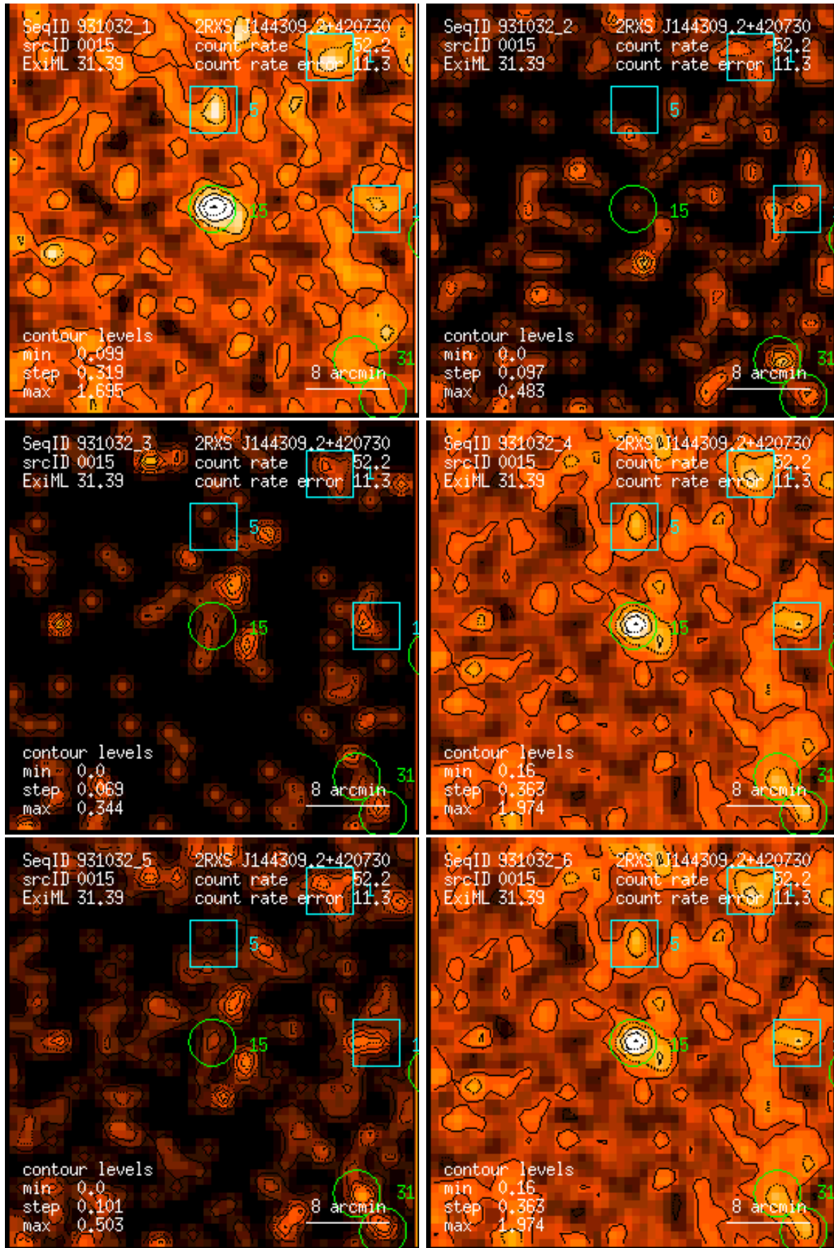
Figure 15: RASS 931032: detection 0015: band rate images, Gaussian filter: (1) PSPC channels 11 – 41, (2) 52 – 90, (3) 91 – 201, (4) 11 – 235, (5) 52 – 201, (6) 11 – 201. Broad band rates in counts/ks. Band rate contour levels in counts/ks/arcmin 2 .
