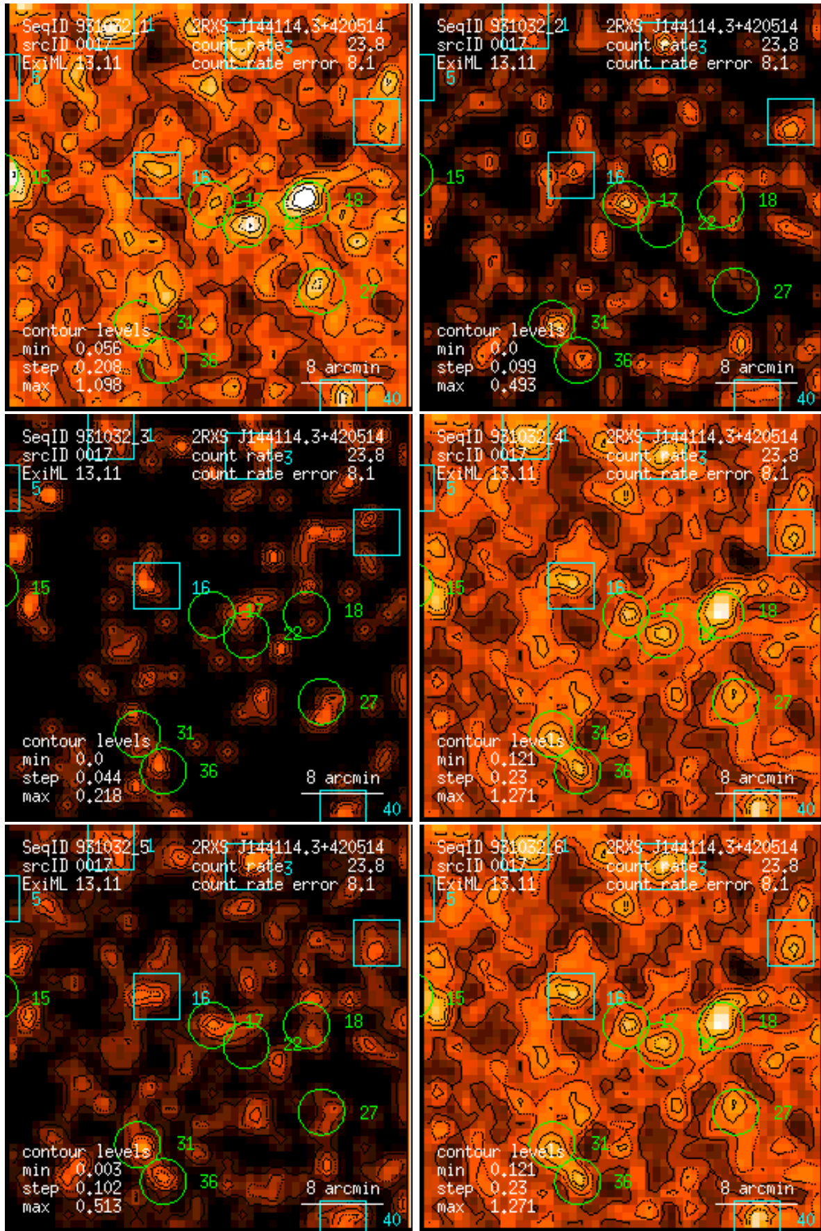
Figure 17: RASS 931032: detection 0017: band rate images, Gaussian filter: (1) PSPC channels 11 – 41, (2) 52 – 90, (3) 91 – 201, (4) 11 – 235, (5) 52 – 201, (6) 11 – 201. Broad band rates in counts/ks. Band rate contour levels in counts/ks/arcmin 2 .
