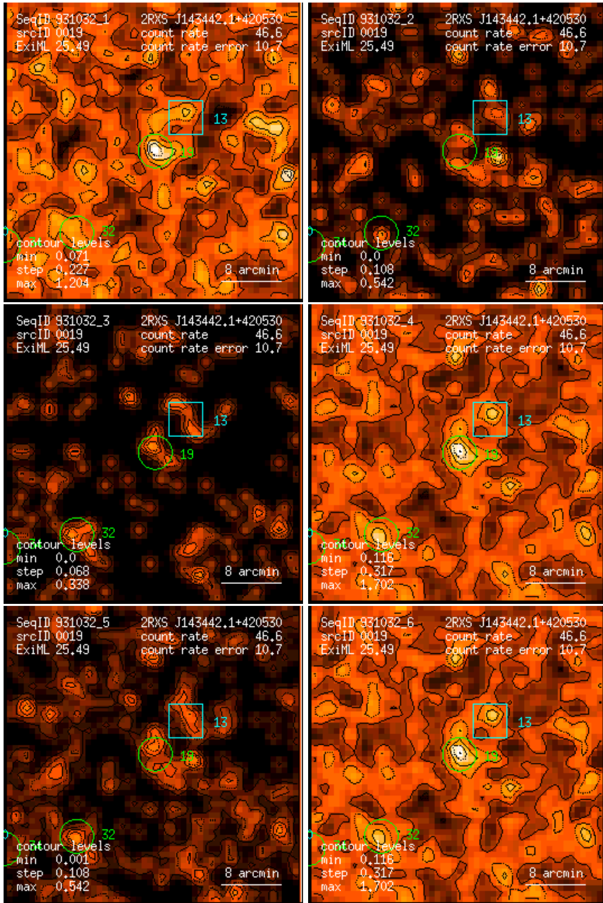
Figure 19: RASS 931032: detection 0019: band rate images, Gaussian filter: (1) PSPC channels 11 – 41, (2) 52 – 90, (3) 91 – 201, (4) 11 – 235, (5) 52 – 201, (6) 11 – 201. Broad band rates in counts/ks. Band rate contour levels in counts/ks/arcmin 2 .
