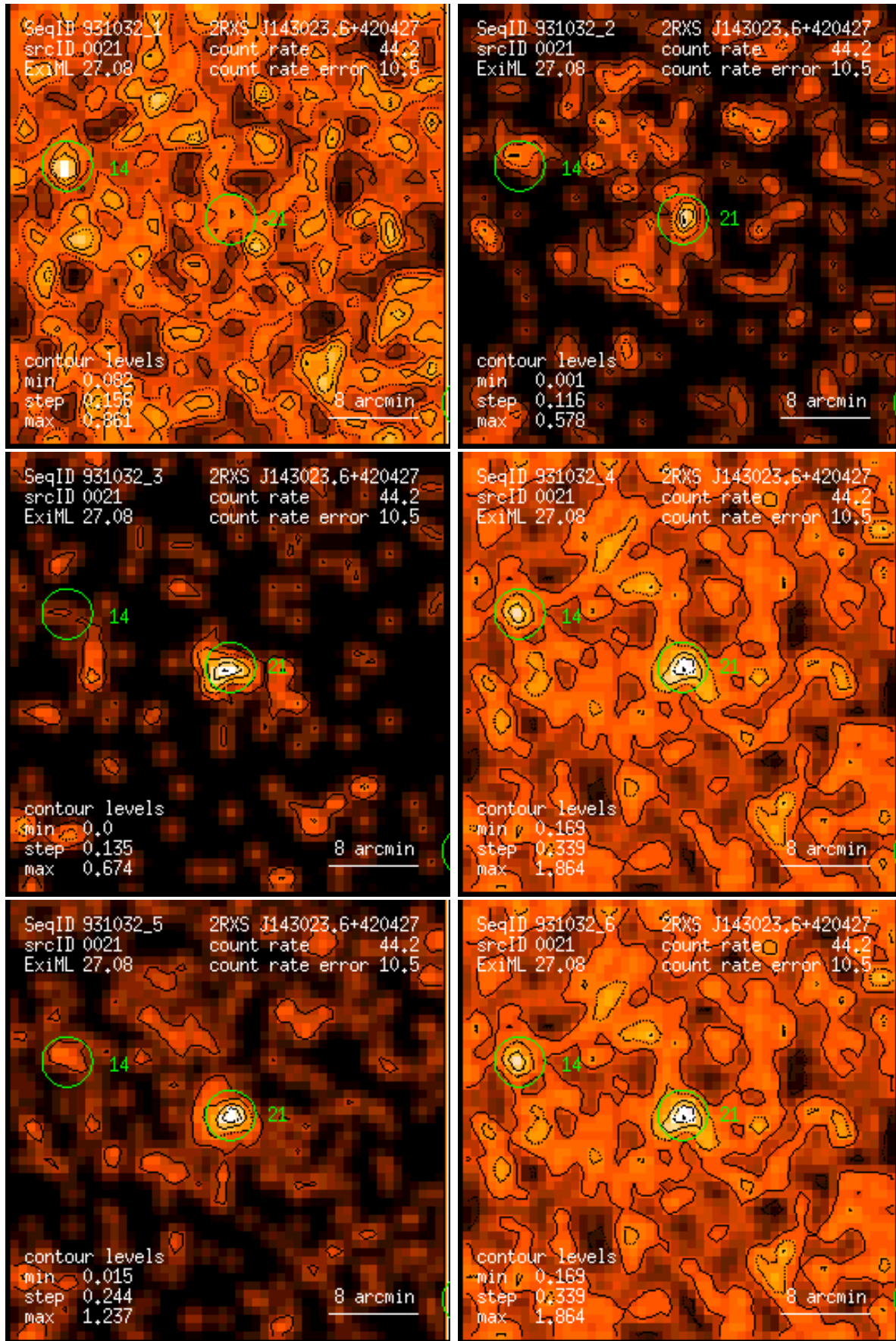
Figure 21: RASS 931032: detection 0021: band rate images, Gaussian filter: (1) PSPC channels 11 – 41, (2) 52 – 90, (3) 91 – 201, (4) 11 – 235, (5) 52 – 201, (6) 11 – 201. Broad band rates in counts/ks. Band rate contour levels in counts/ks/arcmin 2 .
