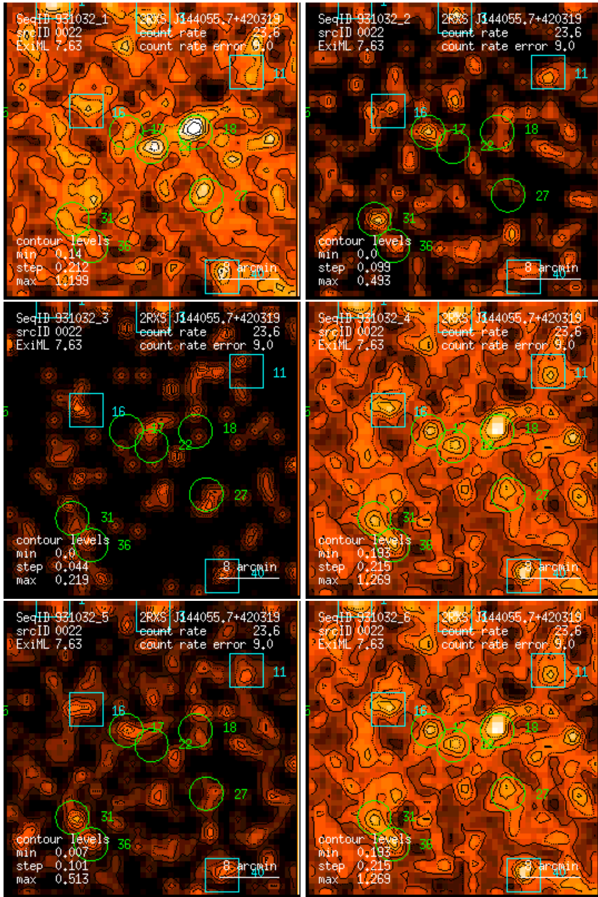
Figure 22: RASS 931032: detection 0022: band rate images, Gaussian filter: (1) PSPC channels 11 – 41, (2) 52 – 90, (3) 91 – 201, (4) 11 – 235, (5) 52 – 201, (6) 11 – 201. Broad band rates in counts/ks. Band rate contour levels in counts/ks/arcmin 2 .
