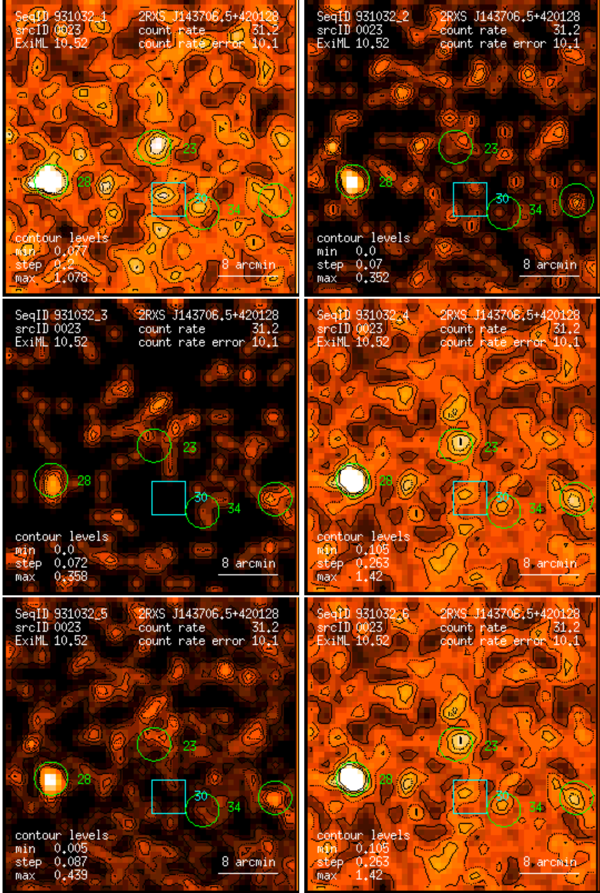
Figure 23: RASS 931032: detection 0023: band rate images, Gaussian filter: (1) PSPC channels 11 – 41, (2) 52 – 90, (3) 91 – 201, (4) 11 – 235, (5) 52 – 201, (6) 11 – 201. Broad band rates in counts/ks. Band rate contour levels in counts/ks/arcmin 2 .
