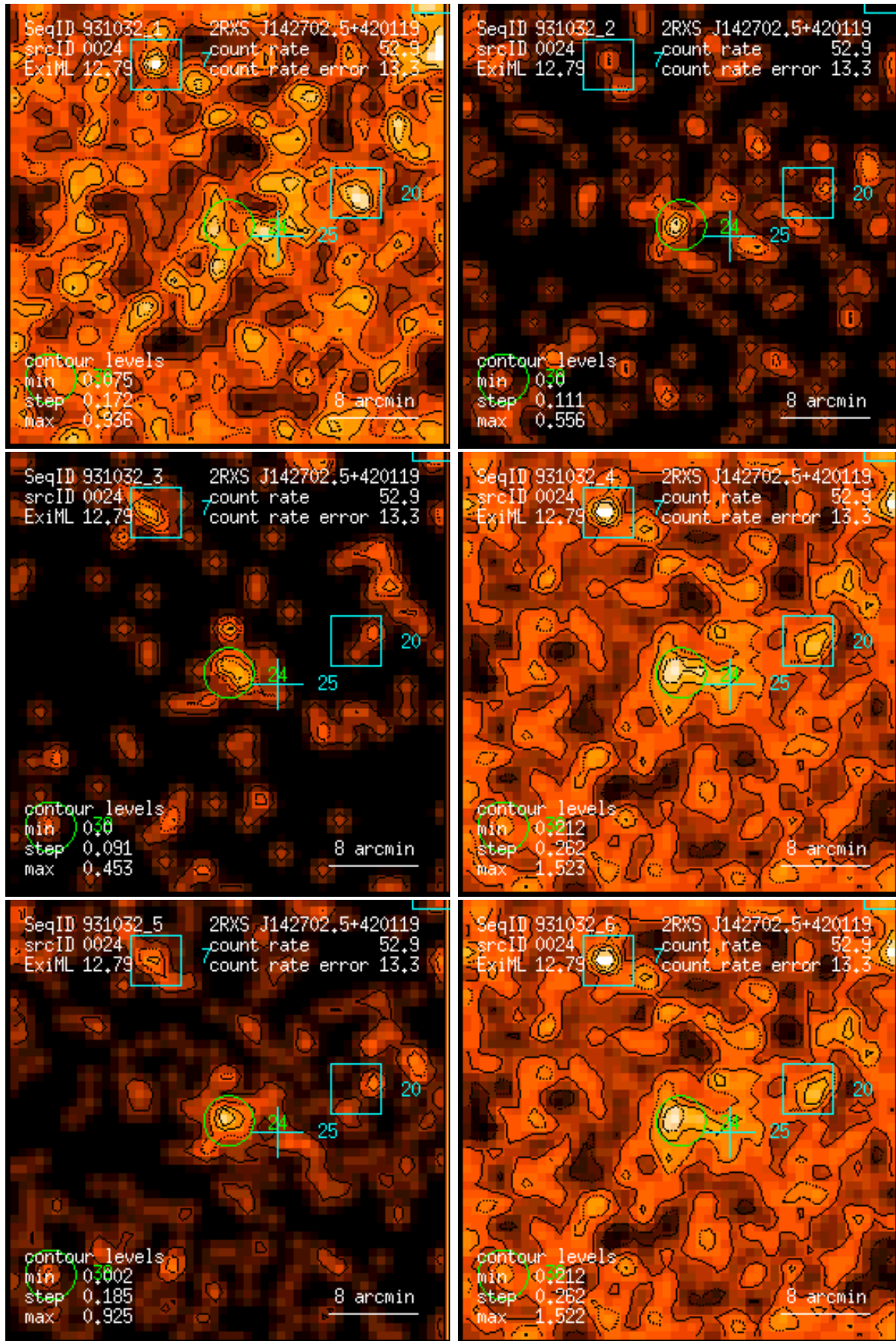
Figure 24: RASS 931032: detection 0024: band rate images, Gaussian filter: (1) PSPC channels 11 – 41, (2) 52 – 90, (3) 91 – 201, (4) 11 – 235, (5) 52 – 201, (6) 11 – 201. Broad band rates in counts/ks. Band rate contour levels in counts/ks/arcmin 2 .
