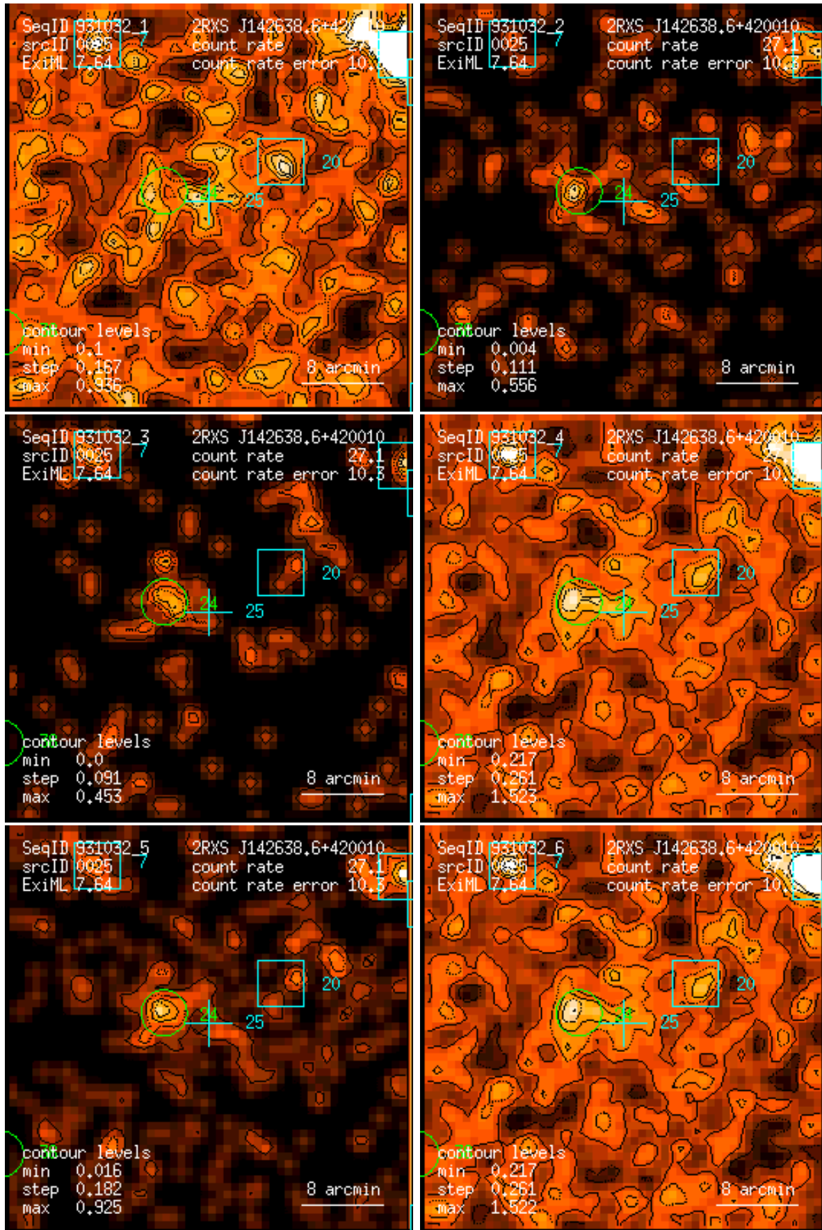
Figure 25: RASS 931032: detection 0025: band rate images, Gaussian filter: (1) PSPC channels 11 – 41, (2) 52 – 90, (3) 91 – 201, (4) 11 – 235, (5) 52 – 201, (6) 11 – 201. Broad band rates in counts/ks. Band rate contour levels in counts/ks/arcmin 2 .
