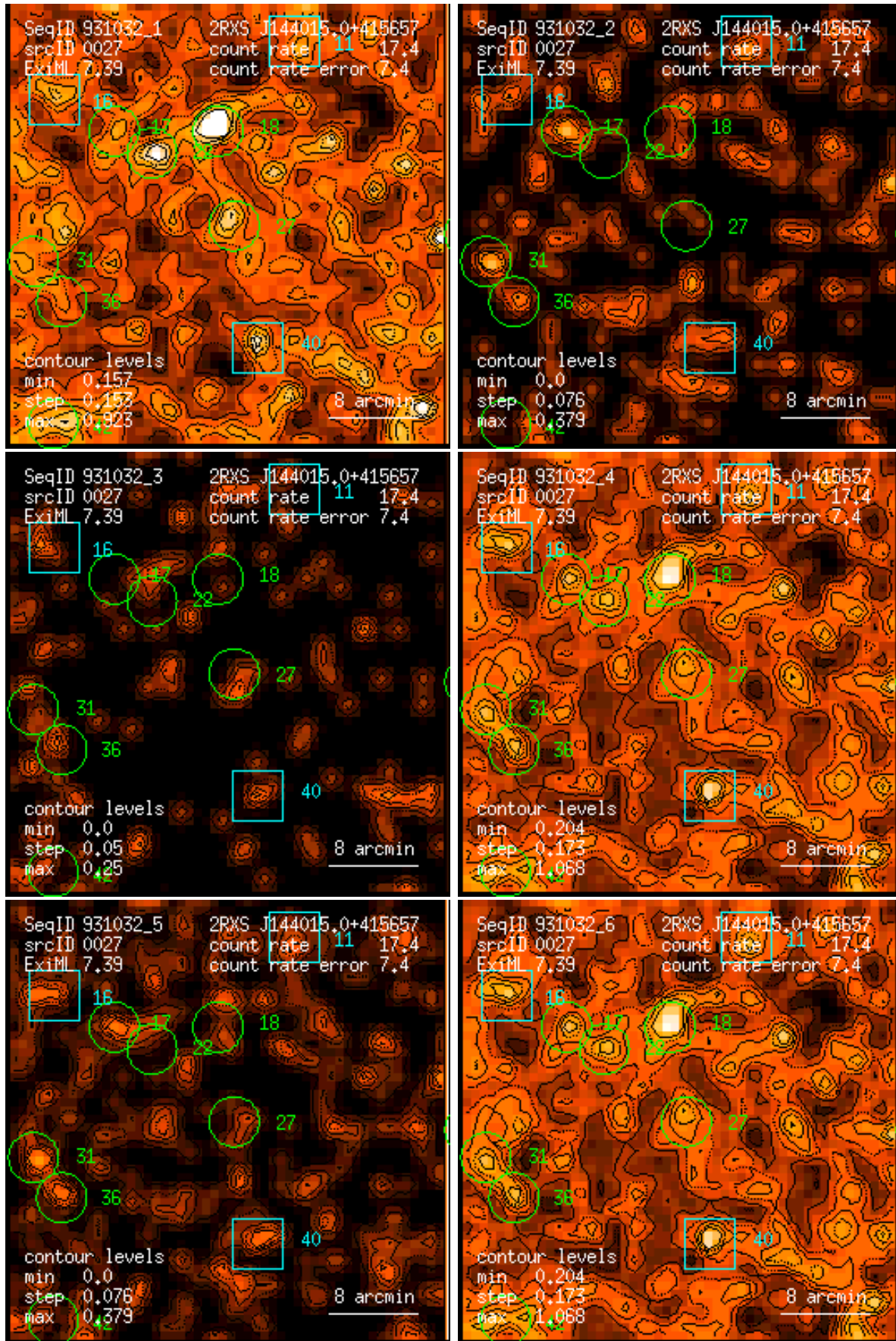
Figure 27: RASS 931032: detection 0027: band rate images, Gaussian filter: (1) PSPC channels 11 – 41, (2) 52 – 90, (3) 91 – 201, (4) 11 – 235, (5) 52 – 201, (6) 11 – 201. Broad band rates in counts/ks. Band rate contour levels in counts/ks/arcmin 2 .
