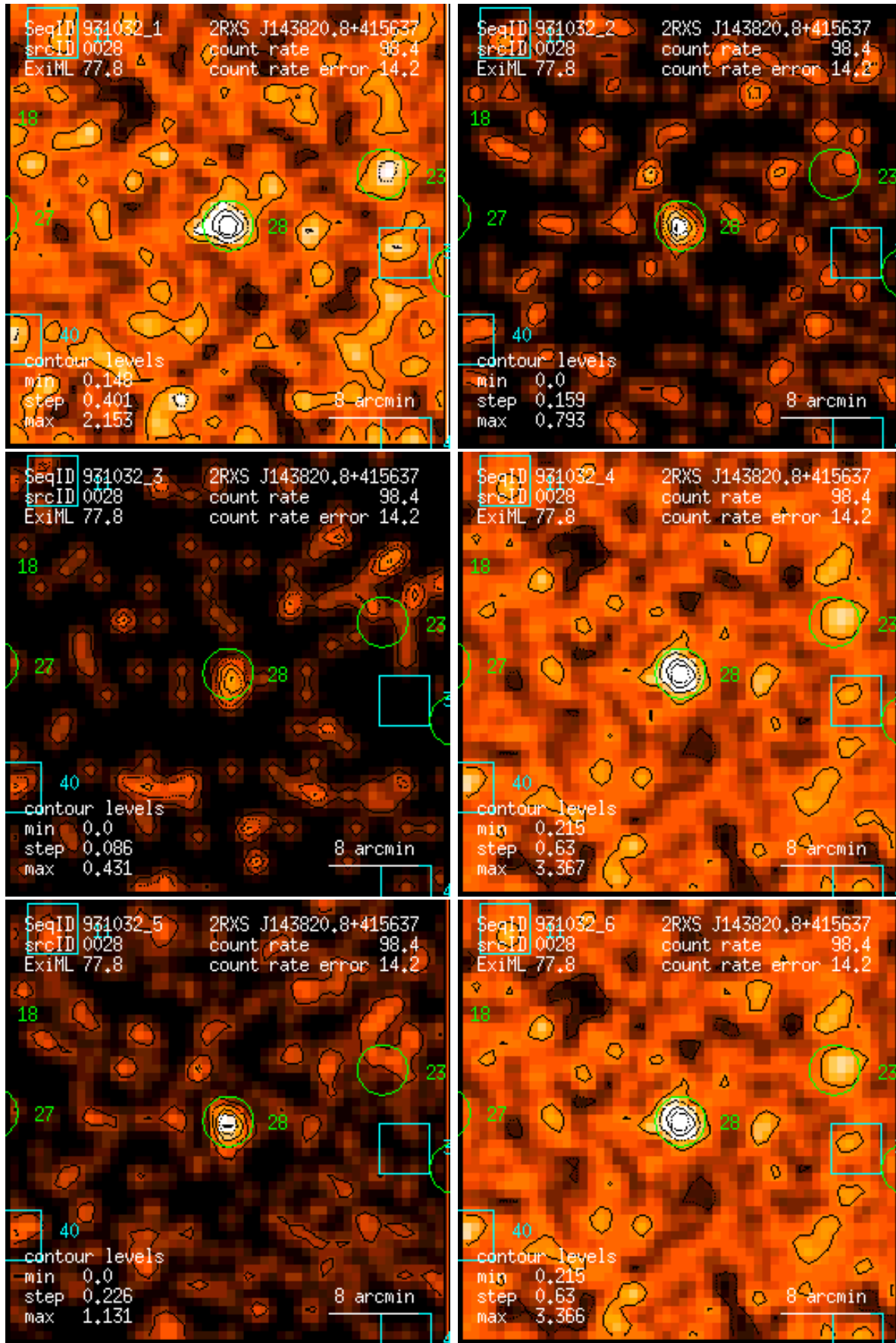
Figure 28: RASS 931032: detection 0028: band rate images, Gaussian filter: (1) PSPC channels 11 – 41, (2) 52 – 90, (3) 91 – 201, (4) 11 – 235, (5) 52 – 201, (6) 11 – 201. Broad band rates in counts/ks. Band rate contour levels in counts/ks/arcmin 2 .
