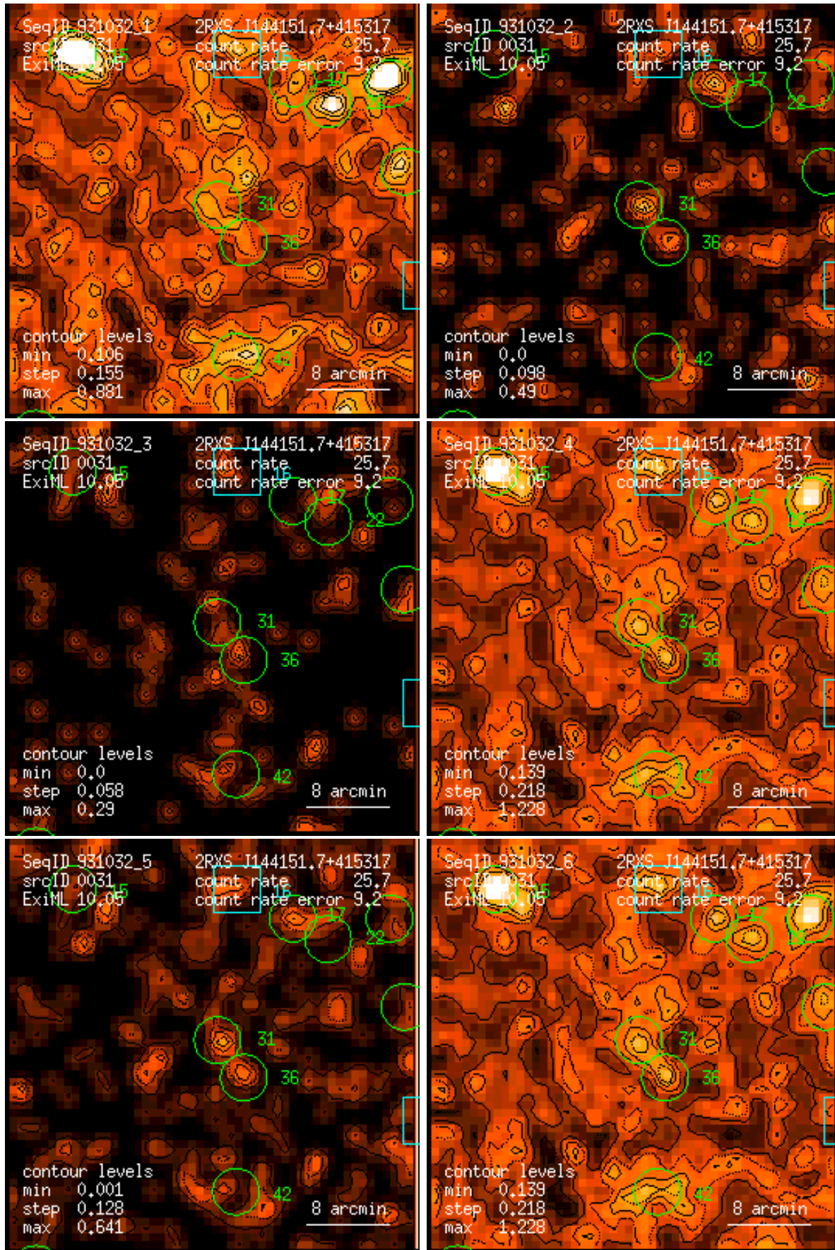
Figure 31: RASS 931032: detection 0031: band rate images, Gaussian filter: (1) PSPC channels 11 – 41, (2) 52 – 90, (3) 91 – 201, (4) 11 – 235, (5) 52 – 201, (6) 11 – 201. Broad band rates in counts/ks. Band rate contour levels in counts/ks/arcmin 2 .
