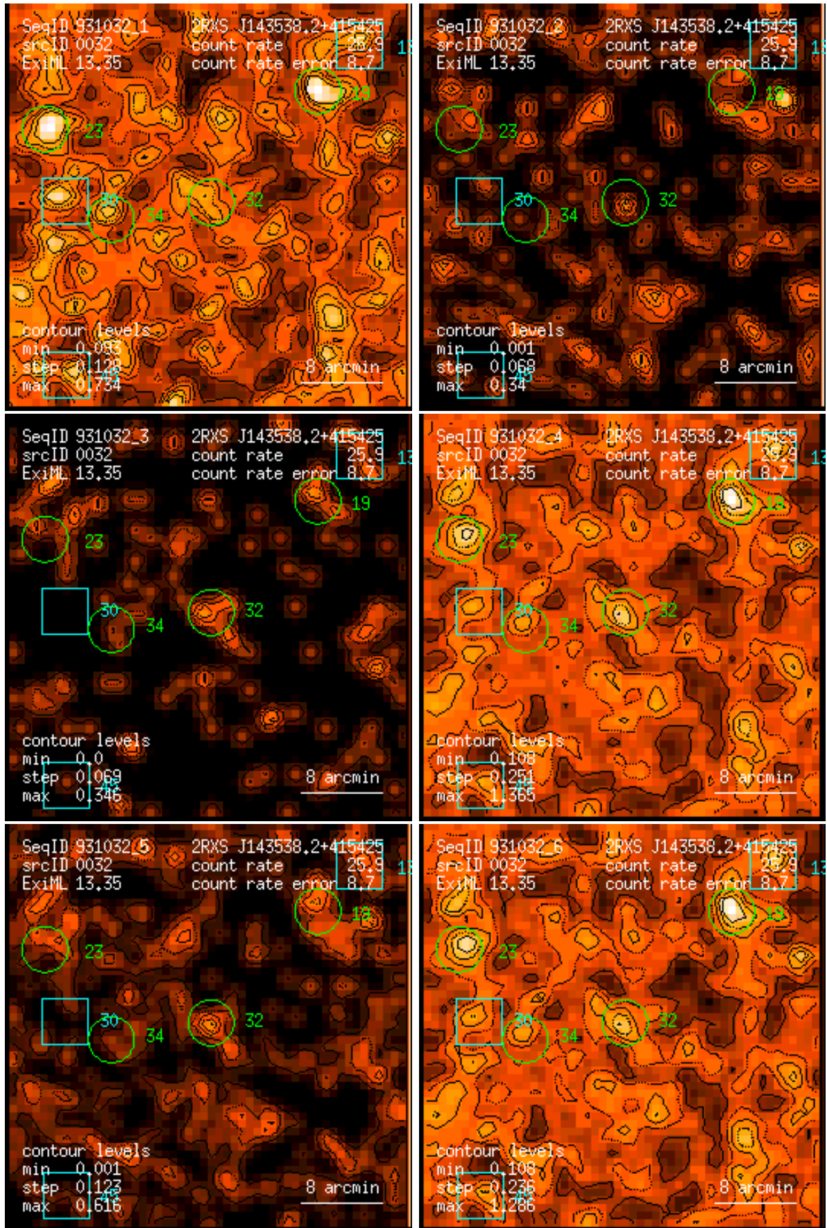
Figure 32: RASS 931032: detection 0032: band rate images, Gaussian filter: (1) PSPC channels 11 – 41, (2) 52 – 90, (3) 91 – 201, (4) 11 – 235, (5) 52 – 201, (6) 11 – 201. Broad band rates in counts/ks. Band rate contour levels in counts/ks/arcmin 2 .
