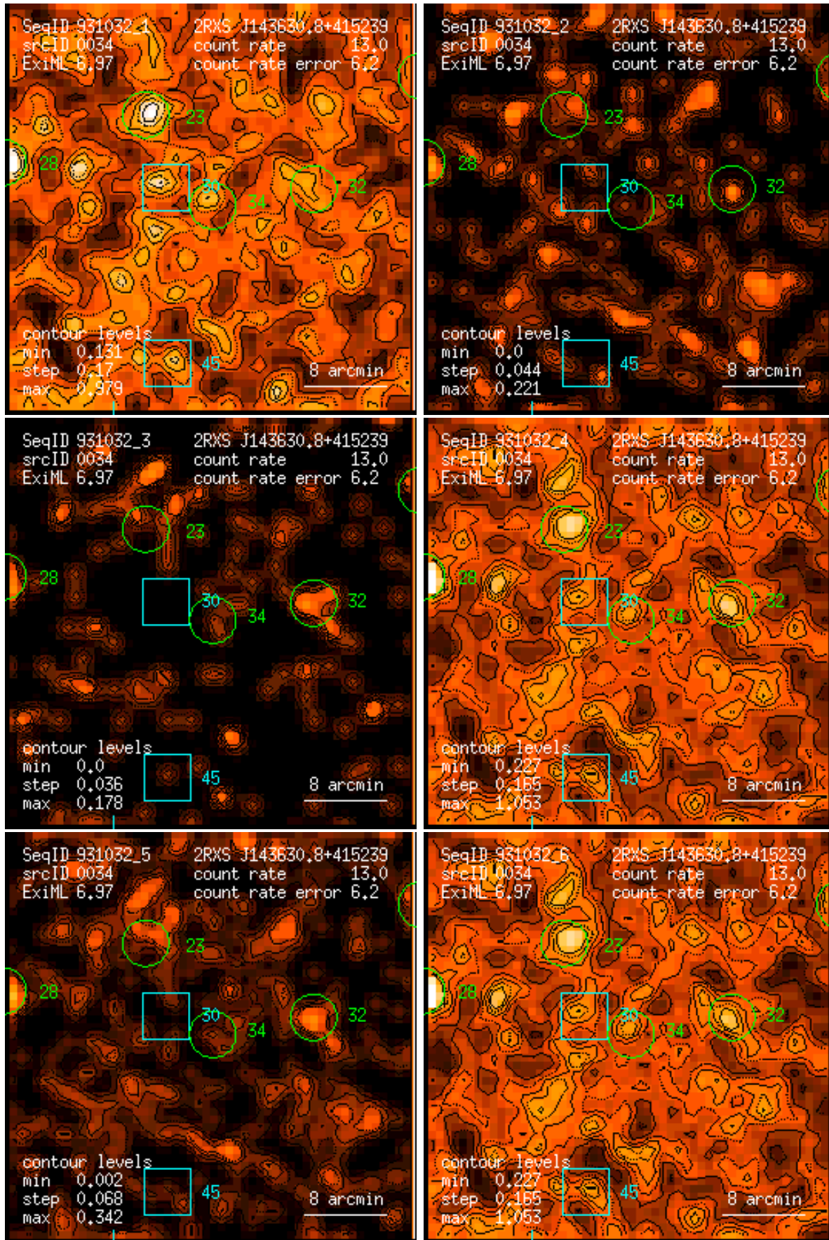
Figure 34: RASS 931032: detection 0034: band rate images, Gaussian filter: (1) PSPC channels 11 – 41, (2) 52 – 90, (3) 91 – 201, (4) 11 – 235, (5) 52 – 201, (6) 11 – 201. Broad band rates in counts/ks. Band rate contour levels in counts/ks/arcmin 2 .
