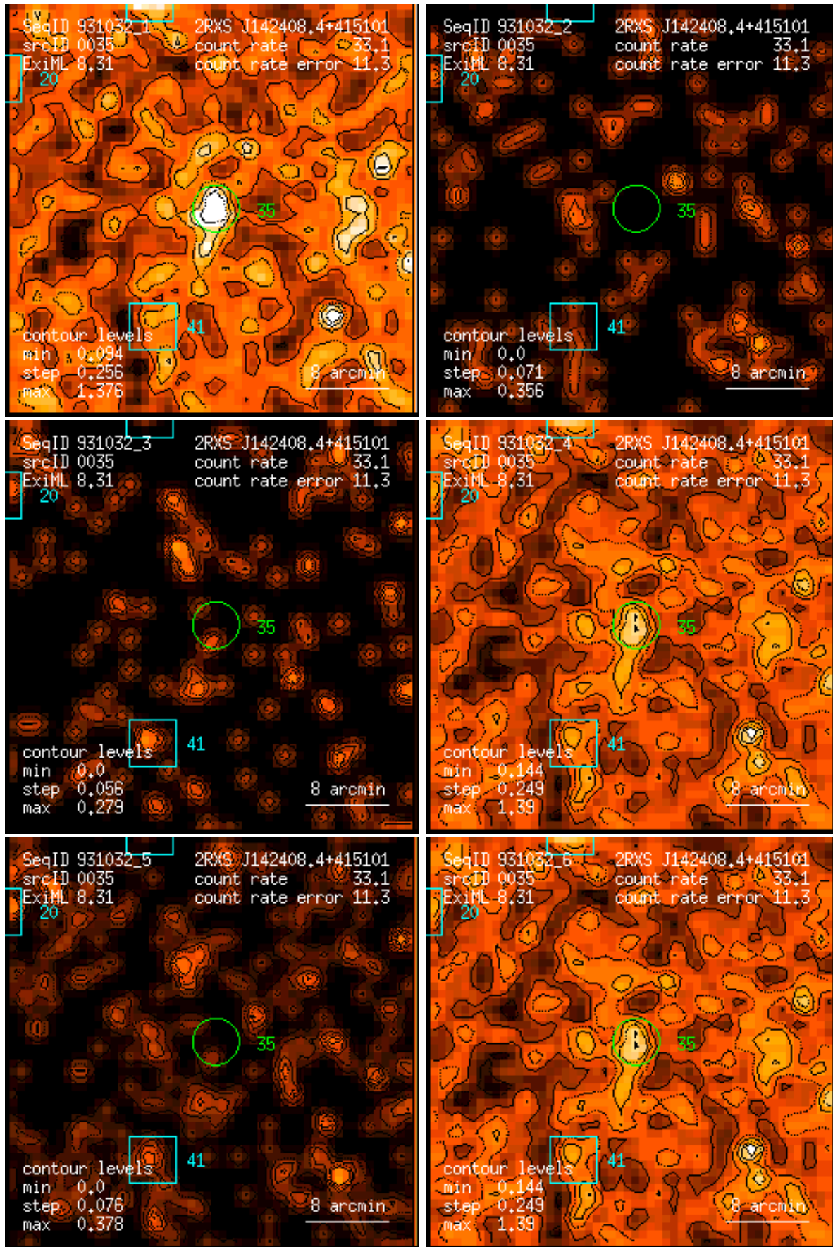
Figure 35: RASS 931032: detection 0035: band rate images, Gaussian filter: (1) PSPC channels 11 – 41, (2) 52 – 90, (3) 91 – 201, (4) 11 – 235, (5) 52 – 201, (6) 11 – 201. Broad band rates in counts/ks. Band rate contour levels in counts/ks/arcmin 2 .
