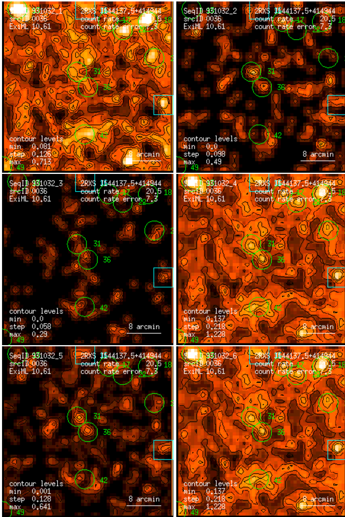
Figure 36: RASS 931032: detection 0036: band rate images, Gaussian filter: (1) PSPC channels 11 – 41, (2) 52 – 90, (3) 91 – 201, (4) 11 – 235, (5) 52 – 201, (6) 11 – 201. Broad band rates in counts/ks. Band rate contour levels in counts/ks/arcmin 2 .
