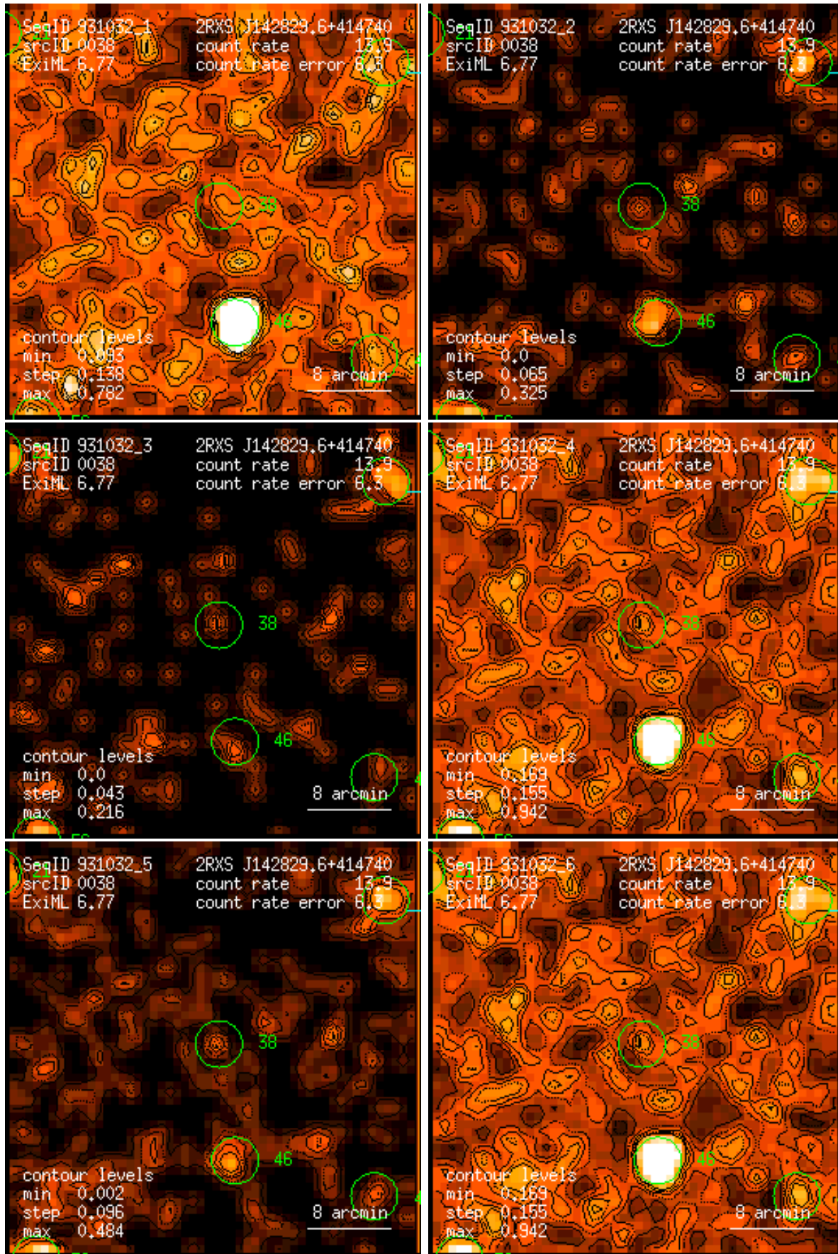
Figure 38: RASS 931032: detection 0038: band rate images, Gaussian filter: (1) PSPC channels 11 – 41, (2) 52 – 90, (3) 91 – 201, (4) 11 – 235, (5) 52 – 201, (6) 11 – 201. Broad band rates in counts/ks. Band rate contour levels in counts/ks/arcmin 2 .
