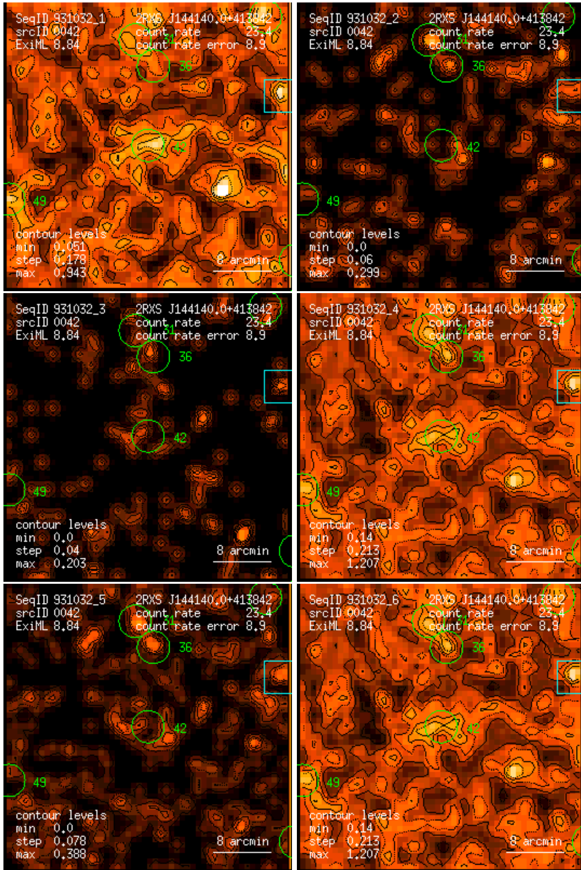
Figure 42: RASS 931032: detection 0042: band rate images, Gaussian filter: (1) PSPC channels 11 – 41, (2) 52 – 90, (3) 91 – 201, (4) 11 – 235, (5) 52 – 201, (6) 11 – 201. Broad band rates in counts/ks. Band rate contour levels in counts/ks/arcmin 2 .
