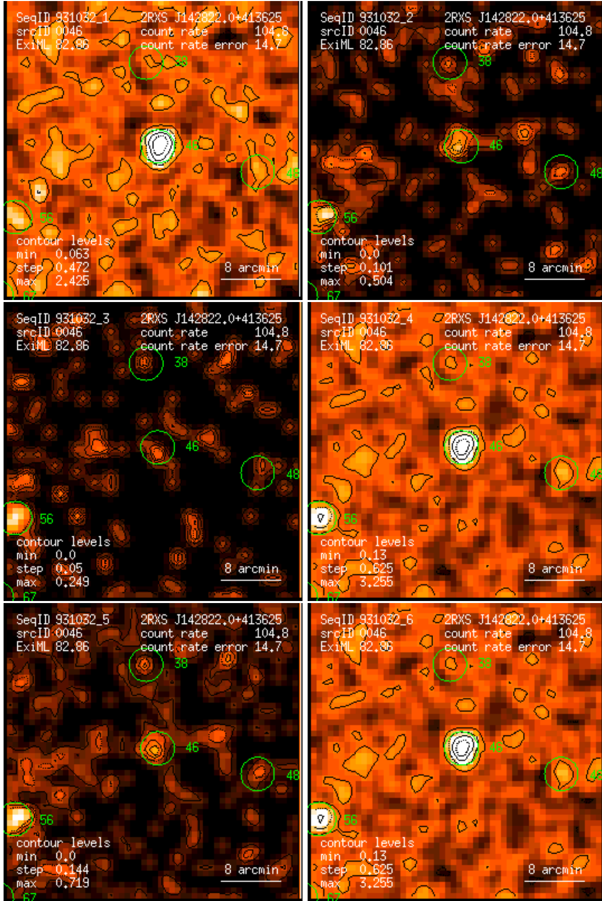
Figure 46: RASS 931032: detection 0046: band rate images, Gaussian filter: (1) PSPC channels 11 – 41, (2) 52 – 90, (3) 91 – 201, (4) 11 – 235, (5) 52 – 201, (6) 11 – 201. Broad band rates in counts/ks. Band rate contour levels in counts/ks/arcmin 2 .
