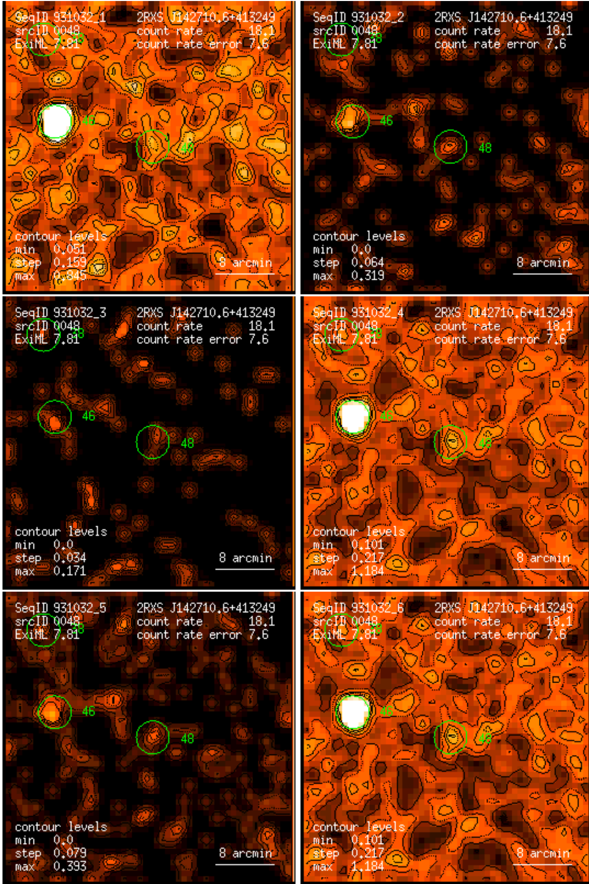
Figure 48: RASS 931032: detection 0048: band rate images, Gaussian filter: (1) PSPC channels 11 – 41, (2) 52 – 90, (3) 91 – 201, (4) 11 – 235, (5) 52 – 201, (6) 11 – 201. Broad band rates in counts/ks. Band rate contour levels in counts/ks/arcmin 2 .
