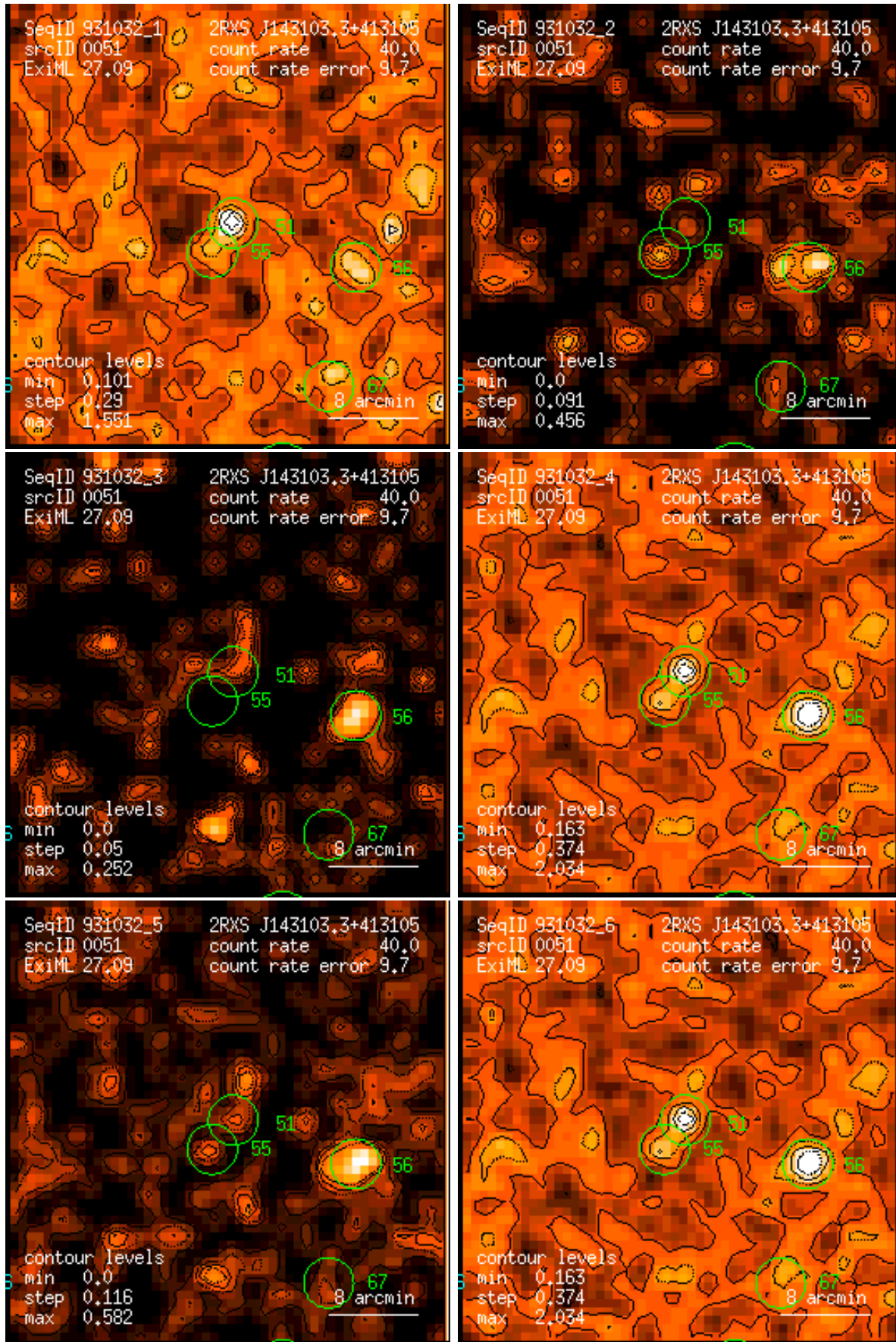
Figure 51: RASS 931032: detection 0051: band rate images, Gaussian filter: (1) PSPC channels 11 – 41, (2) 52 – 90, (3) 91 – 201, (4) 11 – 235, (5) 52 – 201, (6) 11 – 201. Broad band rates in counts/ks. Band rate contour levels in counts/ks/arcmin 2 .
