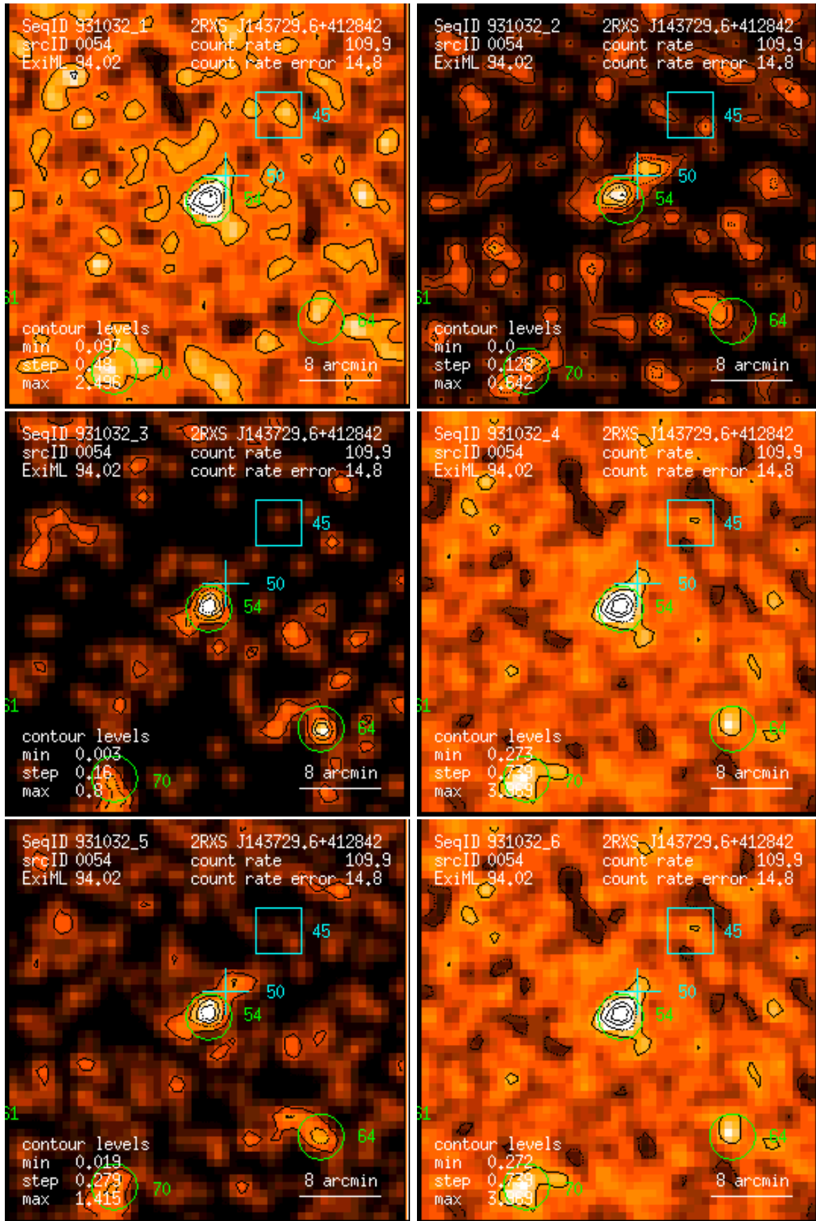
Figure 54: RASS 931032: detection 0054: band rate images, Gaussian filter: (1) PSPC channels 11 – 41, (2) 52 – 90, (3) 91 – 201, (4) 11 – 235, (5) 52 – 201, (6) 11 – 201. Broad band rates in counts/ks. Band rate contour levels in counts/ks/arcmin 2 .
