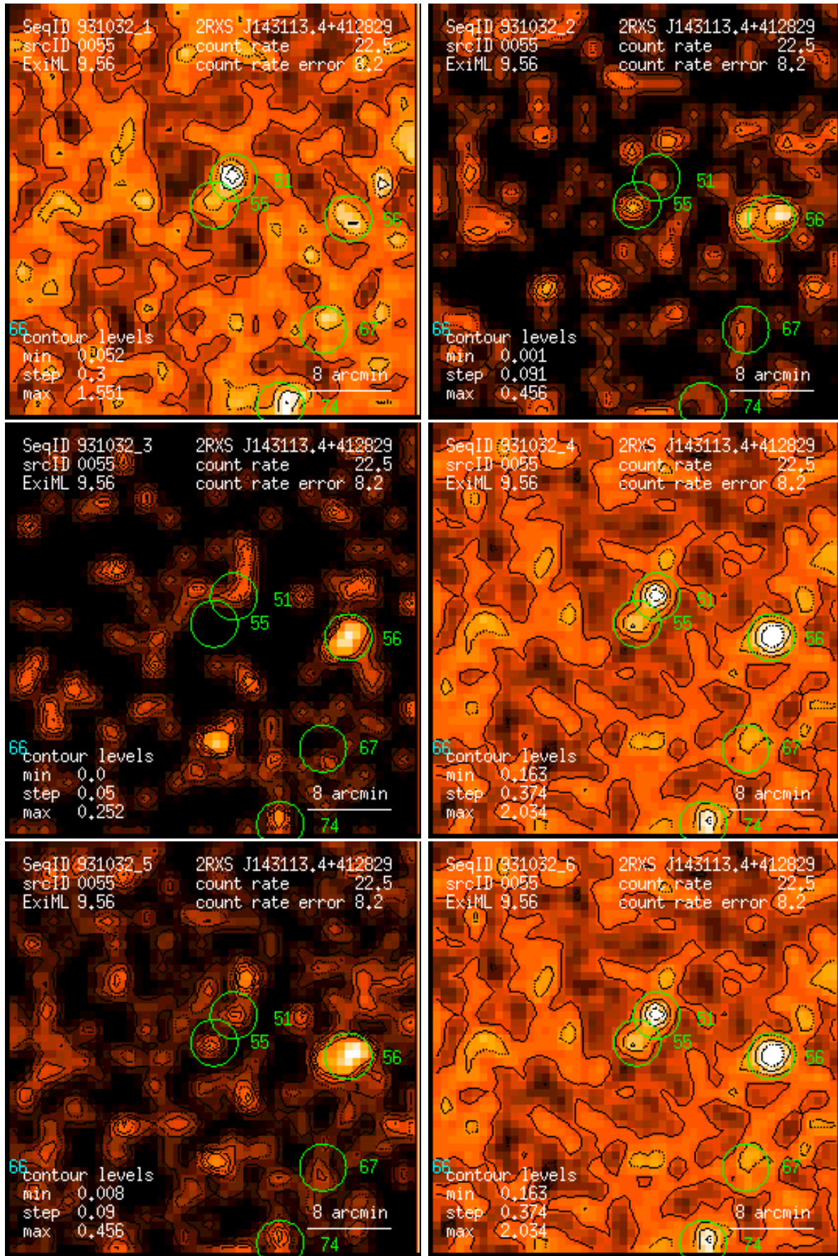
Figure 55: RASS 931032: detection 0055: band rate images, Gaussian filter: (1) PSPC channels 11 – 41, (2) 52 – 90, (3) 91 – 201, (4) 11 – 235, (5) 52 – 201, (6) 11 – 201. Broad band rates in counts/ks. Band rate contour levels in counts/ks/arcmin 2 .
