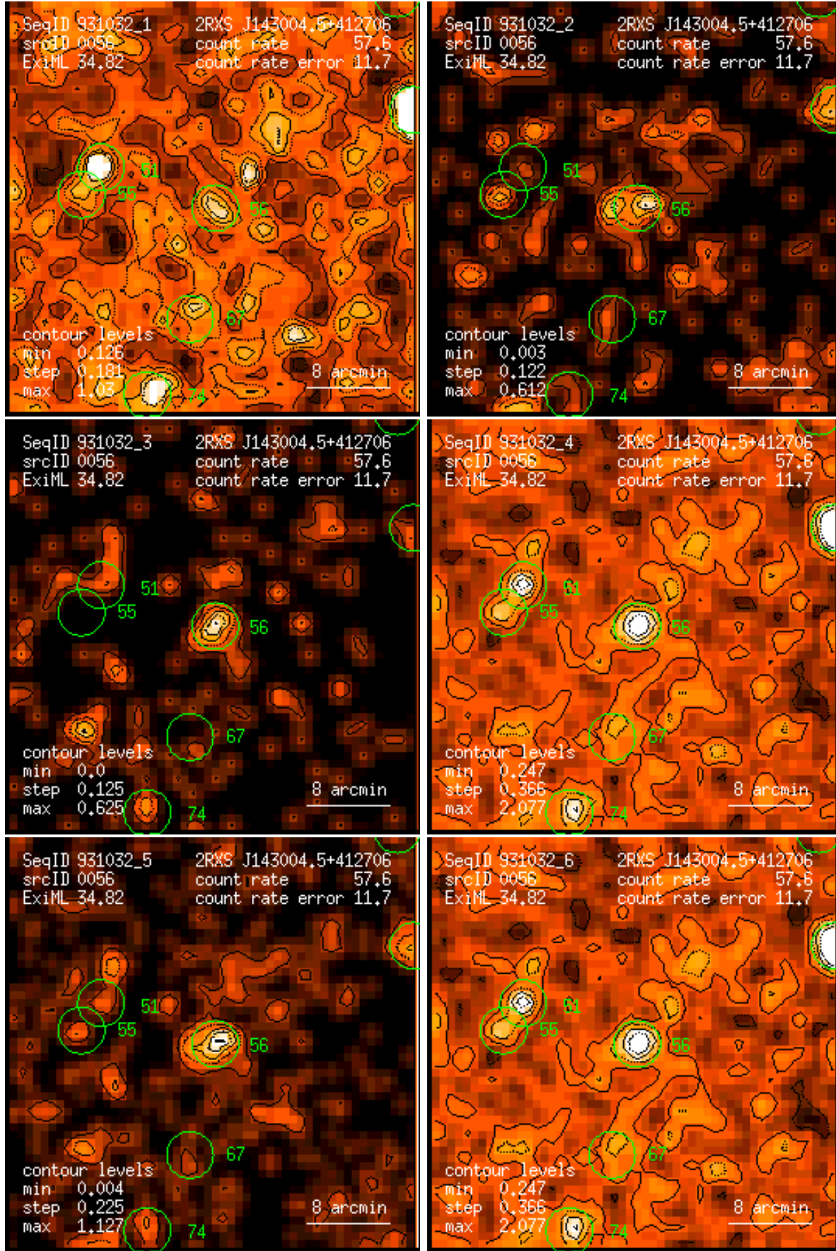
Figure 56: RASS 931032: detection 0056: band rate images, Gaussian filter: (1) PSPC channels 11 – 41, (2) 52 – 90, (3) 91 – 201, (4) 11 – 235, (5) 52 – 201, (6) 11 – 201. Broad band rates in counts/ks. Band rate contour levels in counts/ks/arcmin 2 .
