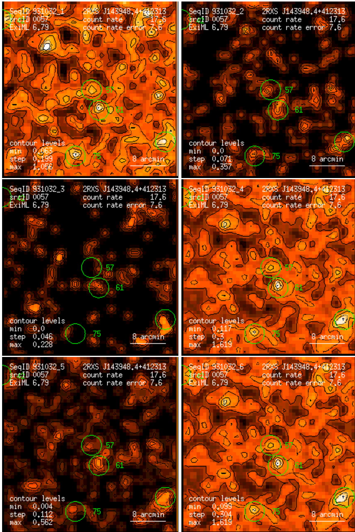
Figure 57: RASS 931032: detection 0057: band rate images, Gaussian filter: (1) PSPC channels 11 – 41, (2) 52 – 90, (3) 91 – 201, (4) 11 – 235, (5) 52 – 201, (6) 11 – 201. Broad band rates in counts/ks. Band rate contour levels in counts/ks/arcmin 2 .
