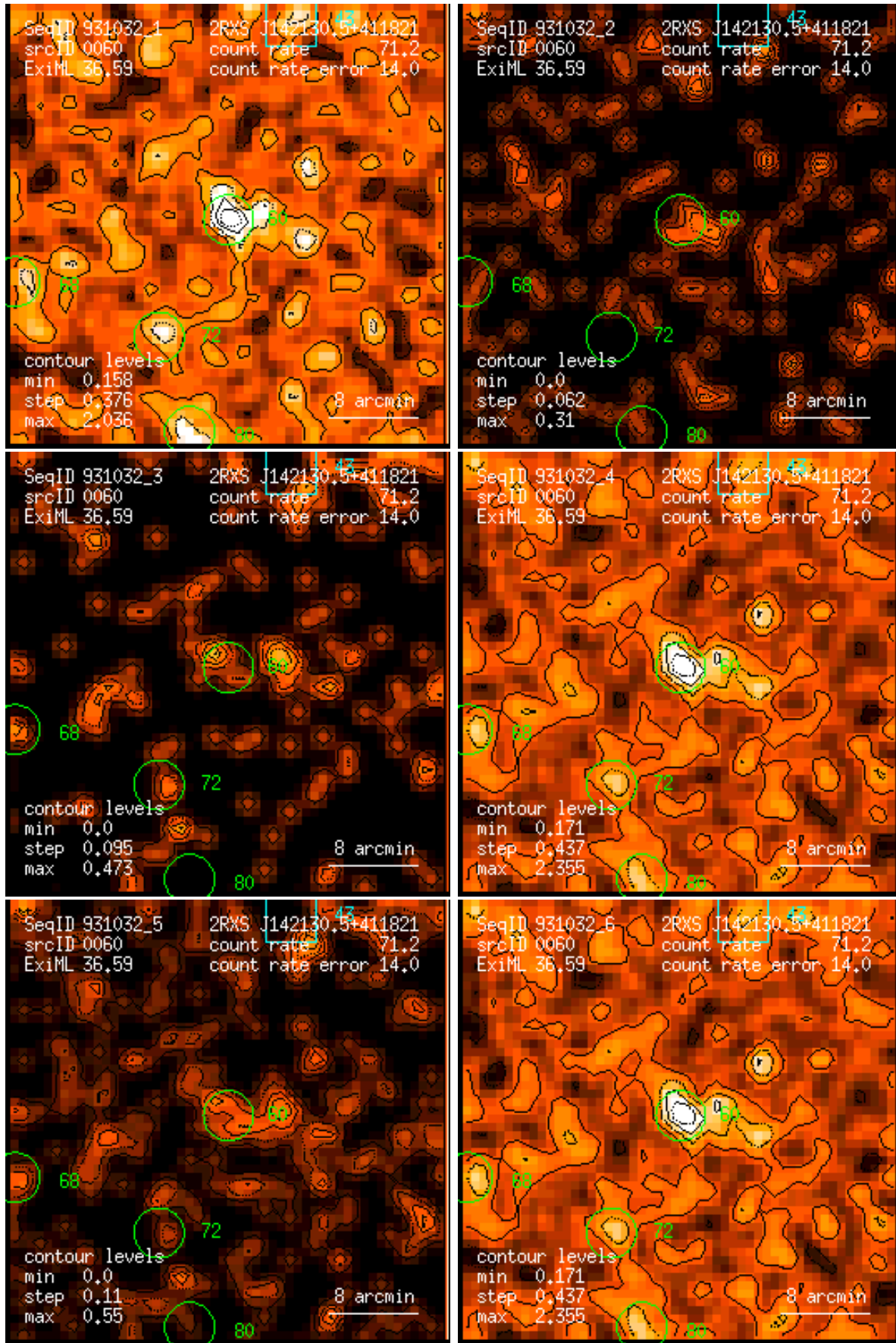
Figure 60: RASS 931032: detection 0060: band rate images, Gaussian filter: (1) PSPC channels 11 – 41, (2) 52 – 90, (3) 91 – 201, (4) 11 – 235, (5) 52 – 201, (6) 11 – 201. Broad band rates in counts/ks. Band rate contour levels in counts/ks/arcmin 2 .
