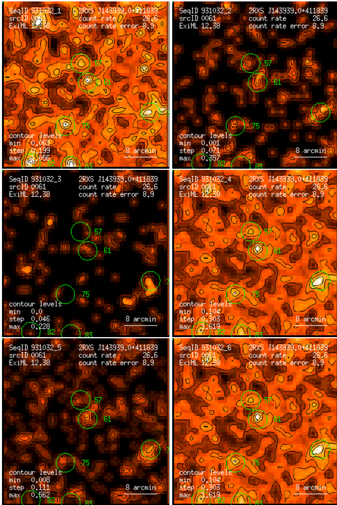
Figure 61: RASS 931032: detection 0061: band rate images, Gaussian filter: (1) PSPC channels 11 – 41, (2) 52 – 90, (3) 91 – 201, (4) 11 – 235, (5) 52 – 201, (6) 11 – 201. Broad band rates in counts/ks. Band rate contour levels in counts/ks/arcmin 2 .
