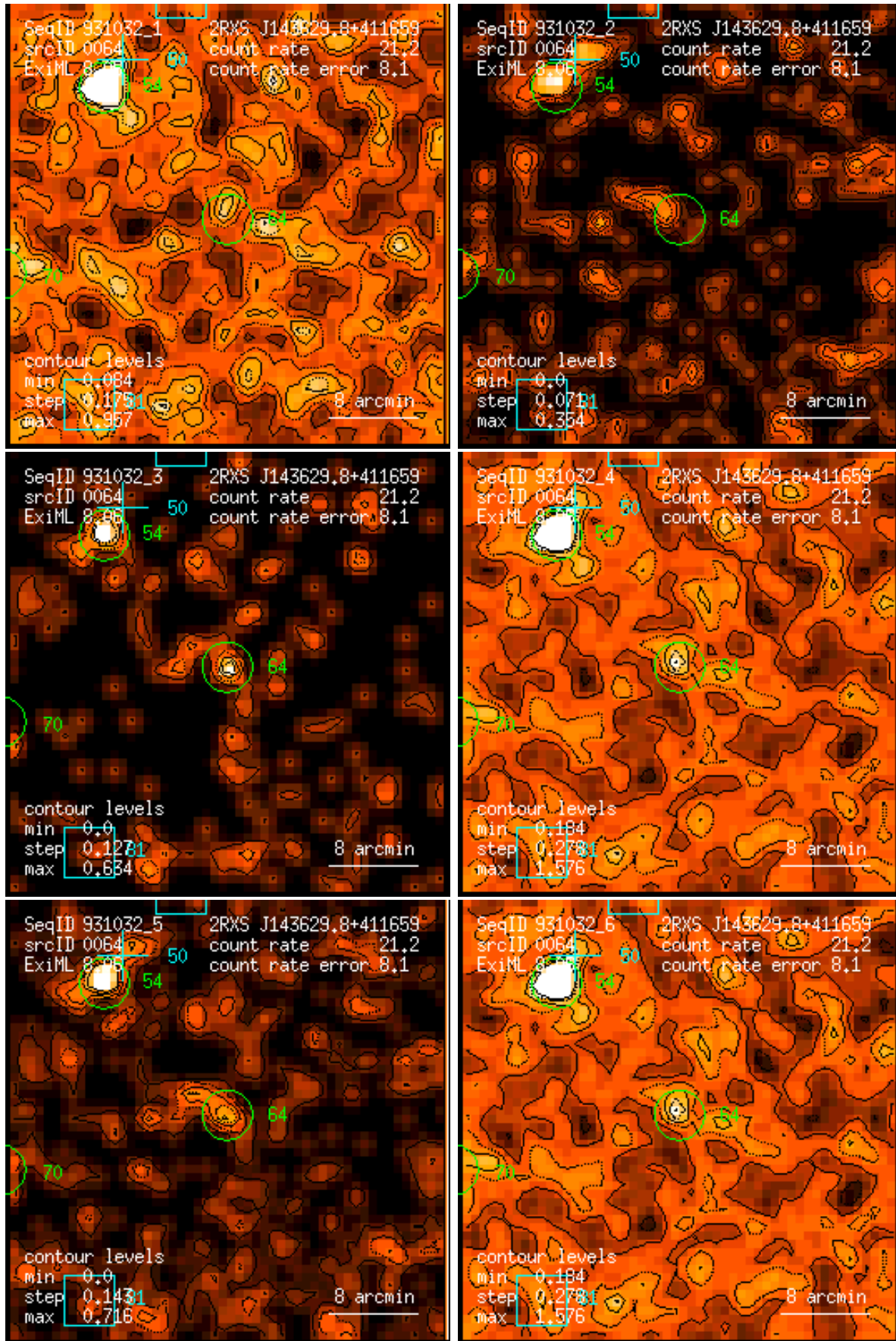
Figure 64: RASS 931032: detection 0064: band rate images, Gaussian filter: (1) PSPC channels 11 – 41, (2) 52 – 90, (3) 91 – 201, (4) 11 – 235, (5) 52 – 201, (6) 11 – 201. Broad band rates in counts/ks. Band rate contour levels in counts/ks/arcmin 2 .
