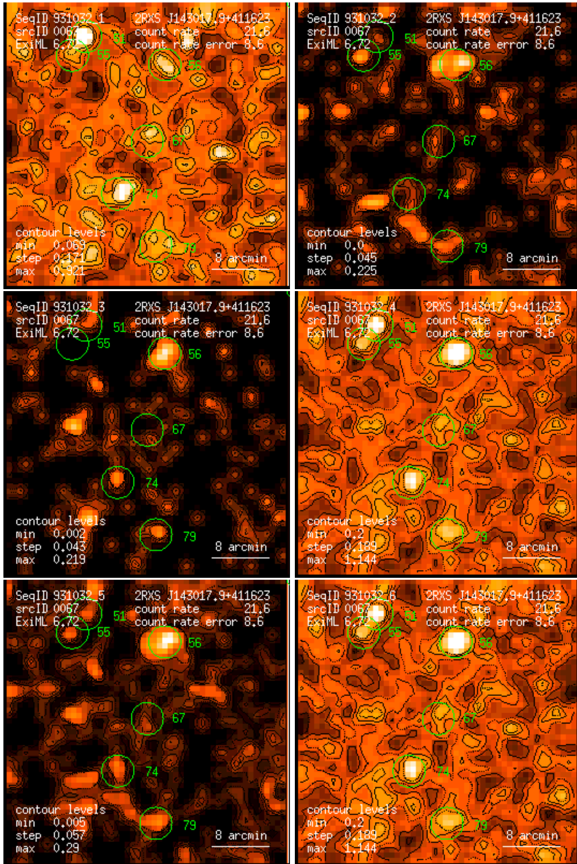
Figure 67: RASS 931032: detection 0067: band rate images, Gaussian filter: (1) PSPC channels 11 – 41, (2) 52 – 90, (3) 91 – 201, (4) 11 – 235, (5) 52 – 201, (6) 11 – 201. Broad band rates in counts/ks. Band rate contour levels in counts/ks/arcmin 2 .
