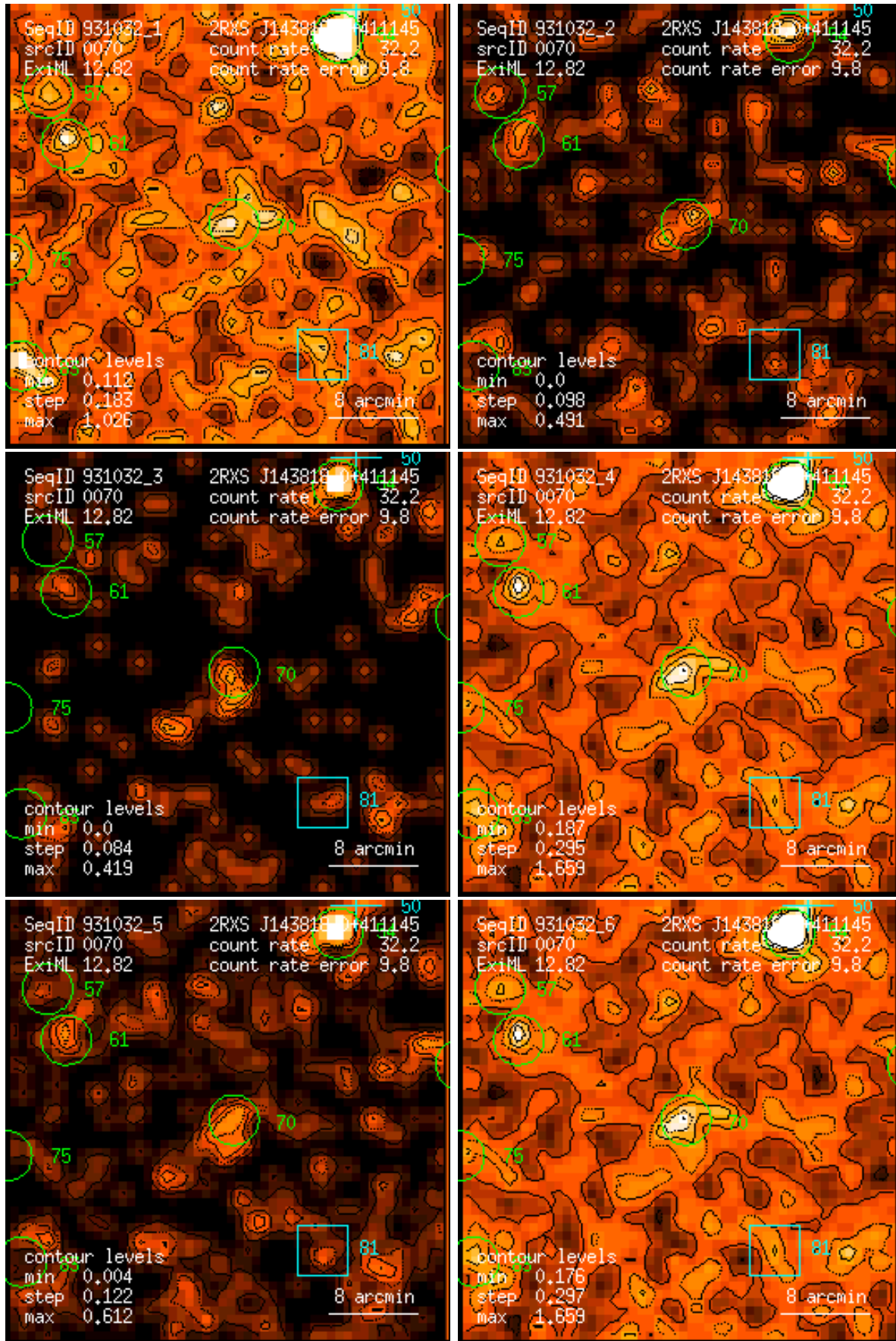
Figure 70: RASS 931032: detection 0070: band rate images, Gaussian filter: (1) PSPC channels 11 – 41, (2) 52 – 90, (3) 91 – 201, (4) 11 – 235, (5) 52 – 201, (6) 11 – 201. Broad band rates in counts/ks. Band rate contour levels in counts/ks/arcmin 2 .
