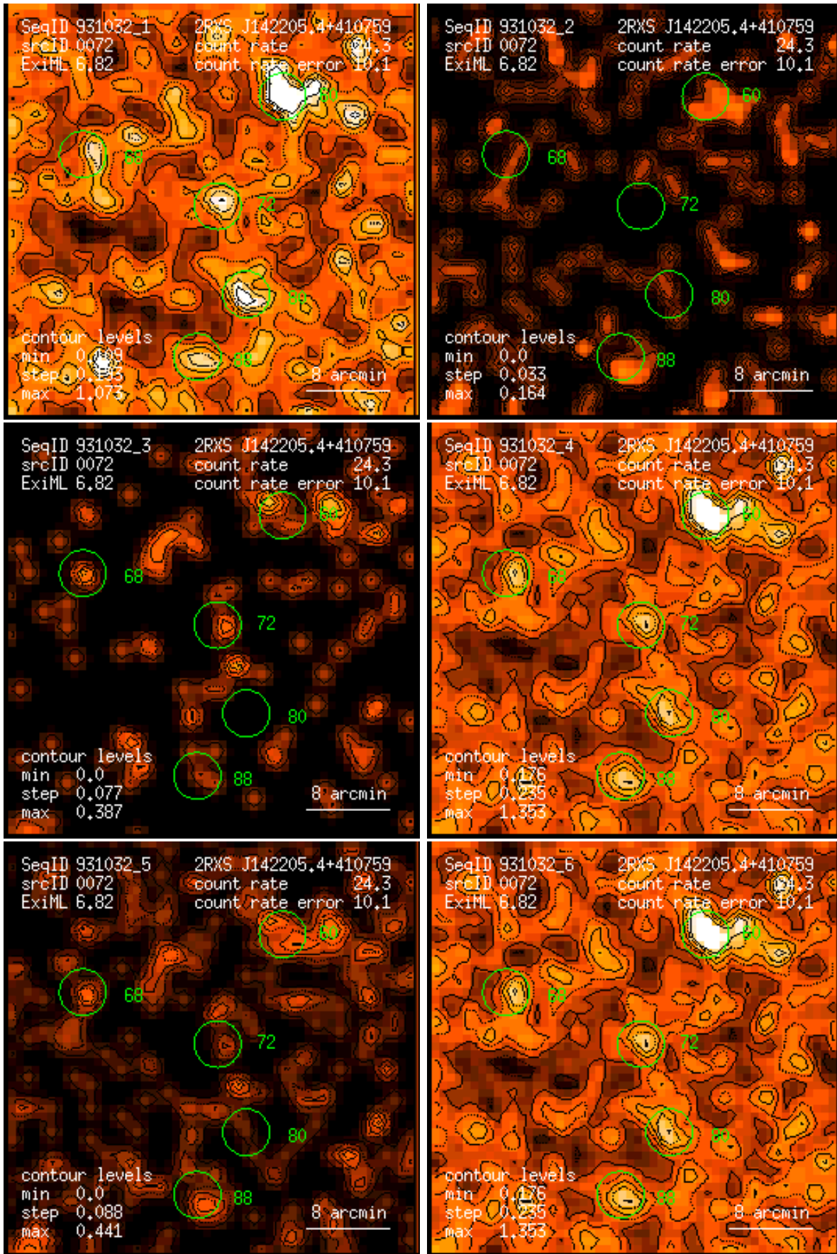
Figure 72: RASS 931032: detection 0072: band rate images, Gaussian filter: (1) PSPC channels 11 – 41, (2) 52 – 90, (3) 91 – 201, (4) 11 – 235, (5) 52 – 201, (6) 11 – 201. Broad band rates in counts/ks. Band rate contour levels in counts/ks/arcmin 2 .
