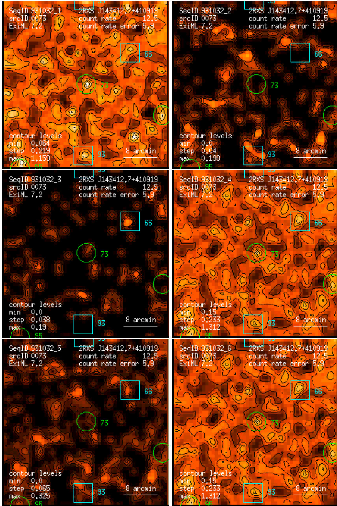
Figure 73: RASS 931032: detection 0073: band rate images, Gaussian filter: (1) PSPC channels 11 – 41, (2) 52 – 90, (3) 91 – 201, (4) 11 – 235, (5) 52 – 201, (6) 11 – 201. Broad band rates in counts/ks. Band rate contour levels in counts/ks/arcmin 2 .
