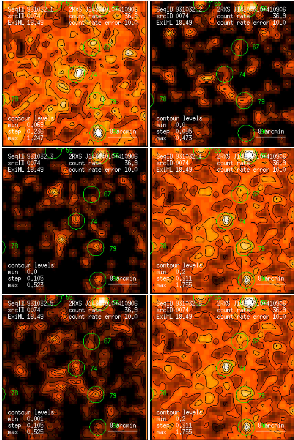
Figure 74: RASS 931032: detection 0074: band rate images, Gaussian filter: (1) PSPC channels 11 – 41, (2) 52 – 90, (3) 91 – 201, (4) 11 – 235, (5) 52 – 201, (6) 11 – 201. Broad band rates in counts/ks. Band rate contour levels in counts/ks/arcmin 2 .
