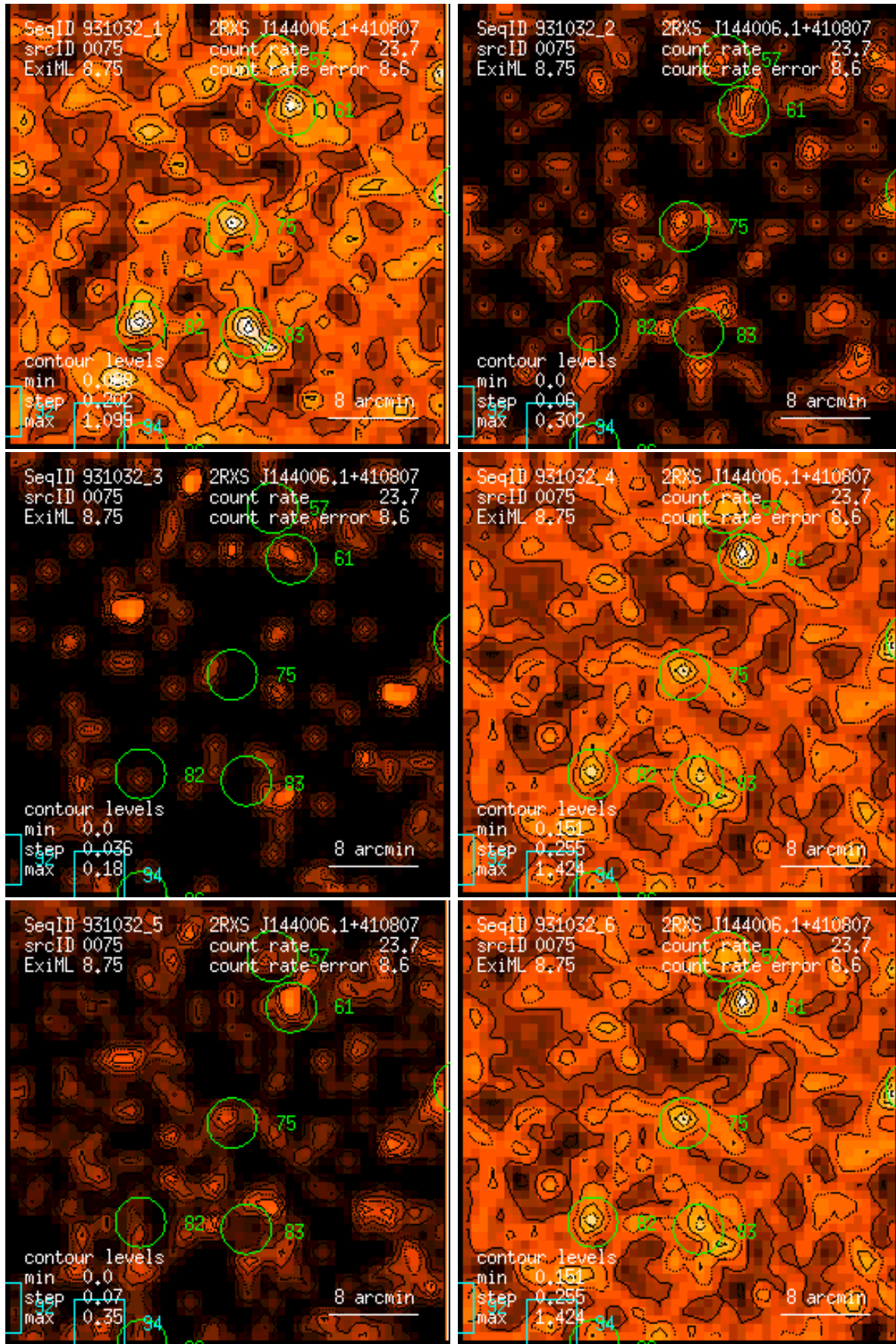
Figure 75: RASS 931032: detection 0075: band rate images, Gaussian filter: (1) PSPC channels 11 – 41, (2) 52 – 90, (3) 91 – 201, (4) 11 – 235, (5) 52 – 201, (6) 11 – 201. Broad band rates in counts/ks. Band rate contour levels in counts/ks/arcmin 2 .
