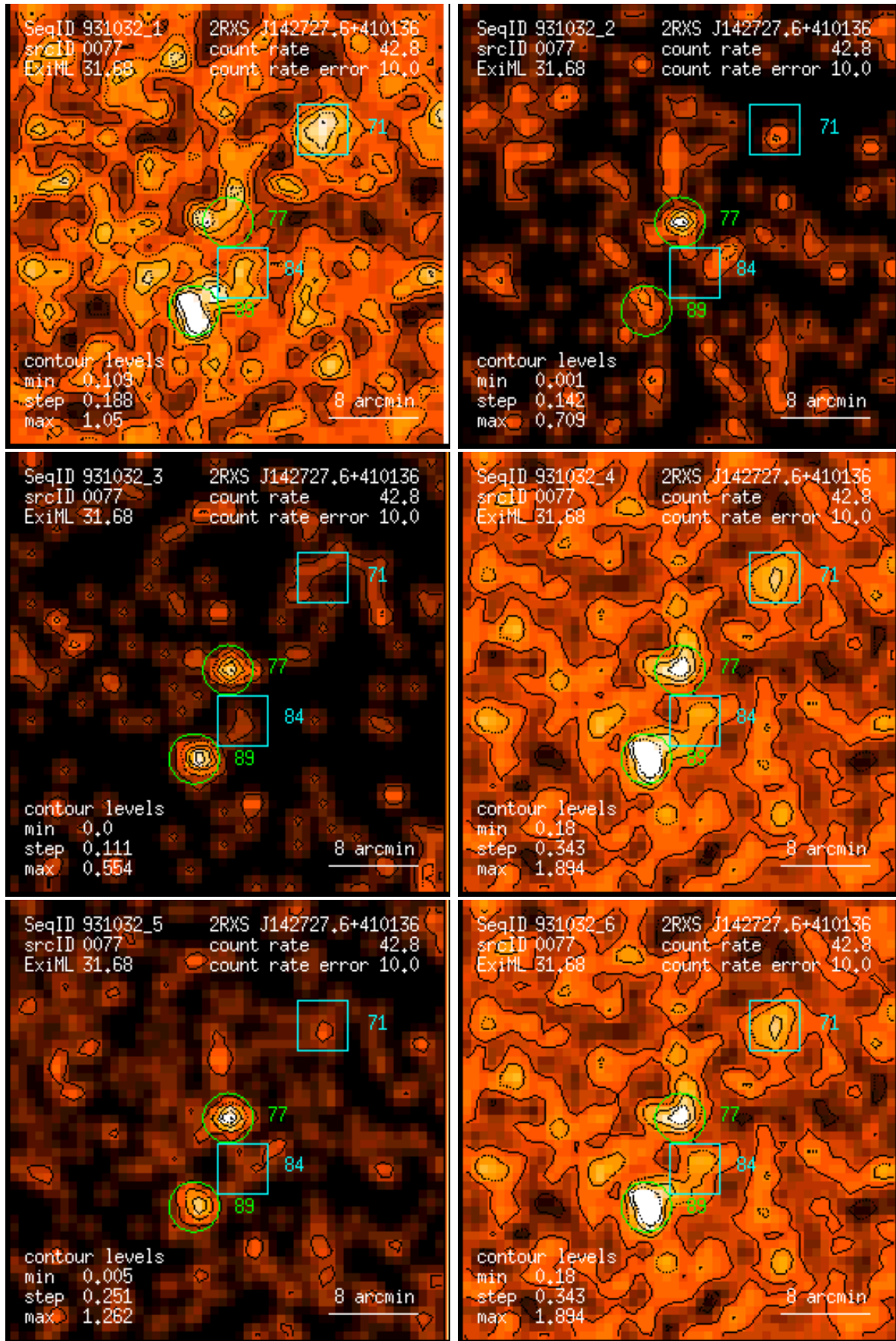
Figure 77: RASS 931032: detection 0077: band rate images, Gaussian filter: (1) PSPC channels 11 – 41, (2) 52 – 90, (3) 91 – 201, (4) 11 – 235, (5) 52 – 201, (6) 11 – 201. Broad band rates in counts/ks. Band rate contour levels in counts/ks/arcmin 2 .
