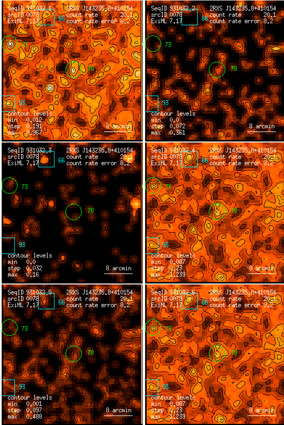
Figure 78: RASS 931032: detection 0078: band rate images, Gaussian filter: (1) PSPC channels 11 – 41, (2) 52 – 90, (3) 91 – 201, (4) 11 – 235, (5) 52 – 201, (6) 11 – 201. Broad band rates in counts/ks. Band rate contour levels in counts/ks/arcmin 2 .
