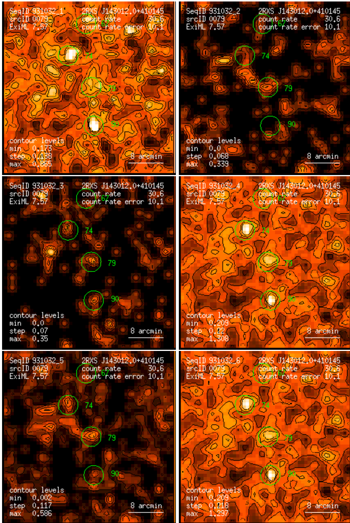
Figure 79: RASS 931032: detection 0079: band rate images, Gaussian filter: (1) PSPC channels 11 – 41, (2) 52 – 90, (3) 91 – 201, (4) 11 – 235, (5) 52 – 201, (6) 11 – 201. Broad band rates in counts/ks. Band rate contour levels in counts/ks/arcmin 2 .
