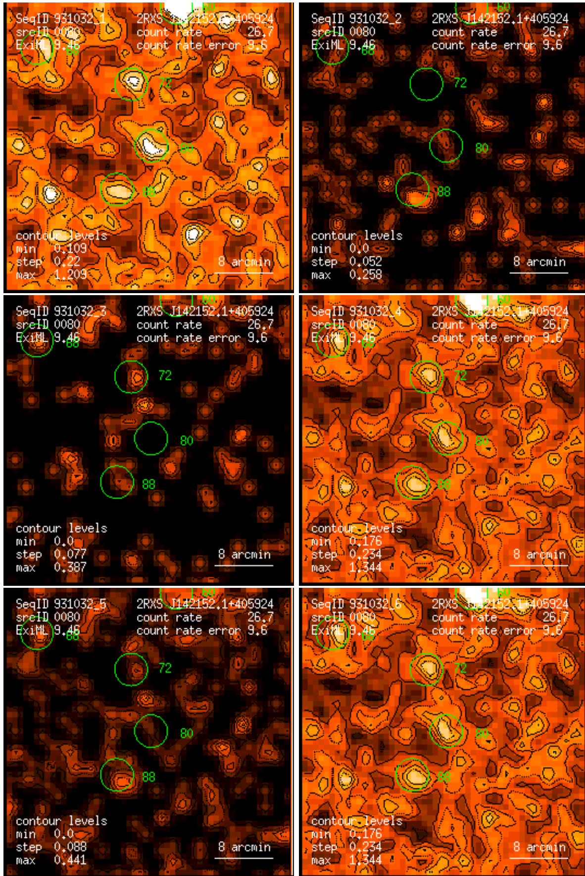
Figure 80: RASS 931032: detection 0080: band rate images, Gaussian filter: (1) PSPC channels 11 – 41, (2) 52 – 90, (3) 91 – 201, (4) 11 – 235, (5) 52 – 201, (6) 11 – 201. Broad band rates in counts/ks. Band rate contour levels in counts/ks/arcmin 2 .
