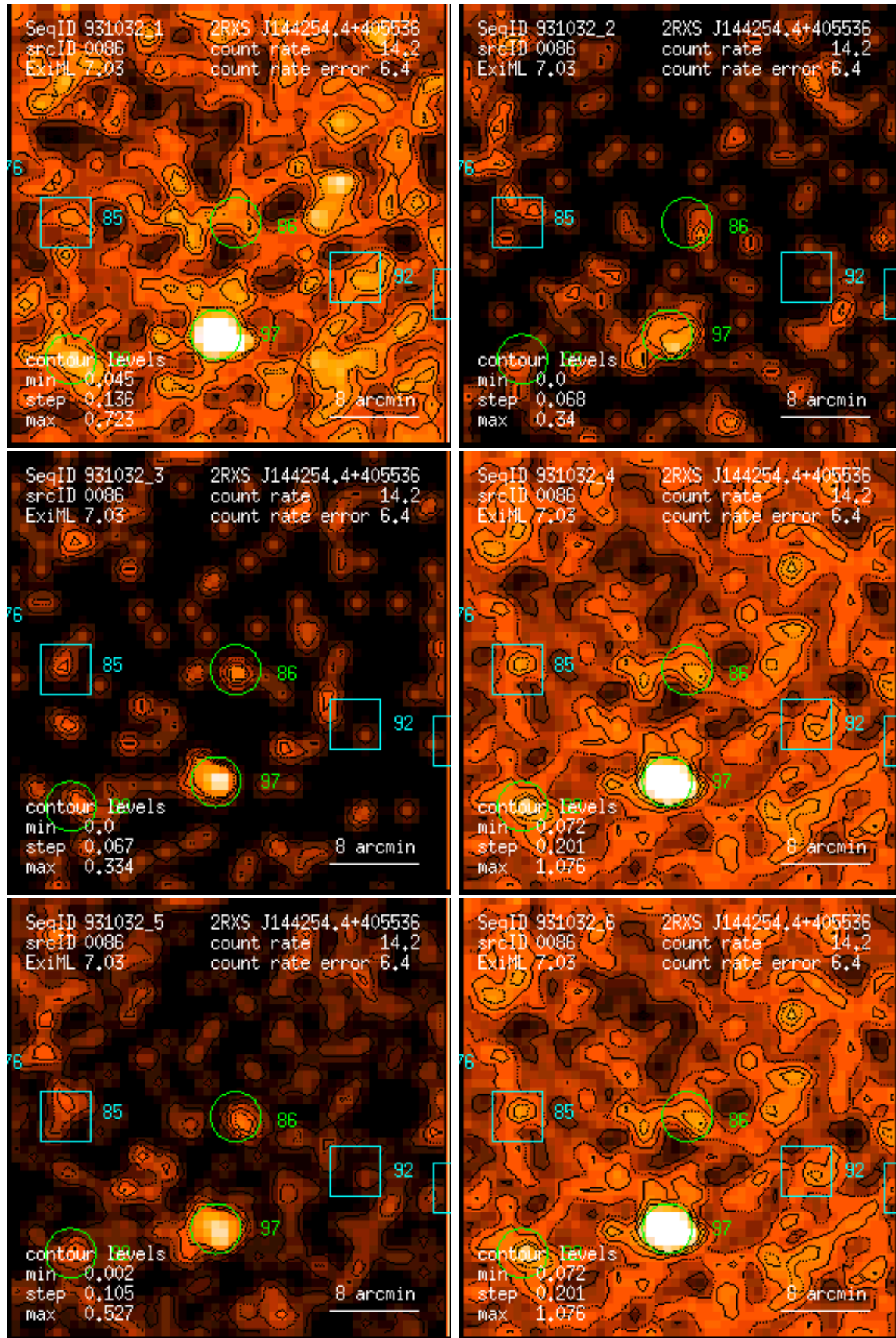
Figure 86: RASS 931032: detection 0086: band rate images, Gaussian filter: (1) PSPC channels 11 – 41, (2) 52 – 90, (3) 91 – 201, (4) 11 – 235, (5) 52 – 201, (6) 11 – 201. Broad band rates in counts/ks. Band rate contour levels in counts/ks/arcmin 2 .
