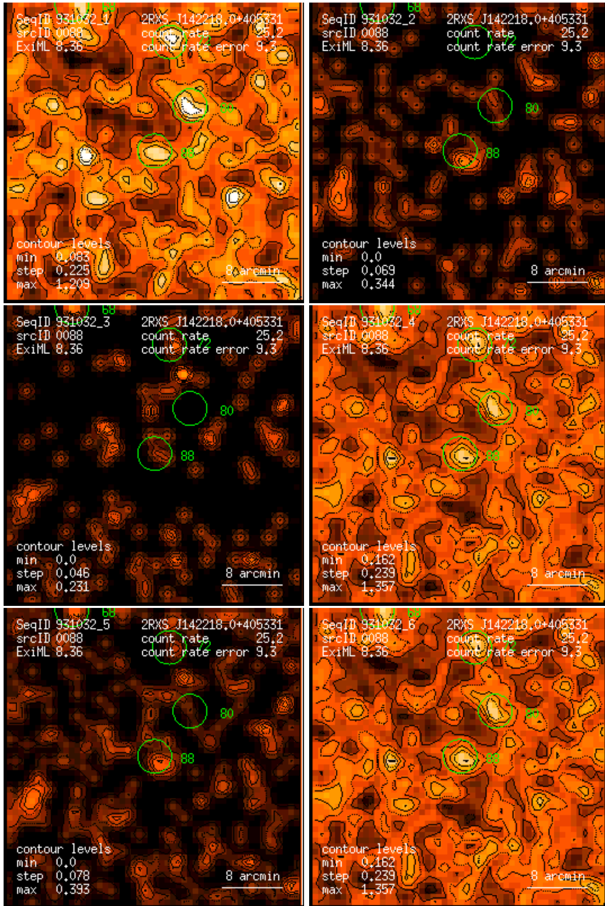
Figure 88: RASS 931032: detection 0088: band rate images, Gaussian filter: (1) PSPC channels 11 – 41, (2) 52 – 90, (3) 91 – 201, (4) 11 – 235, (5) 52 – 201, (6) 11 – 201. Broad band rates in counts/ks. Band rate contour levels in counts/ks/arcmin 2 .
