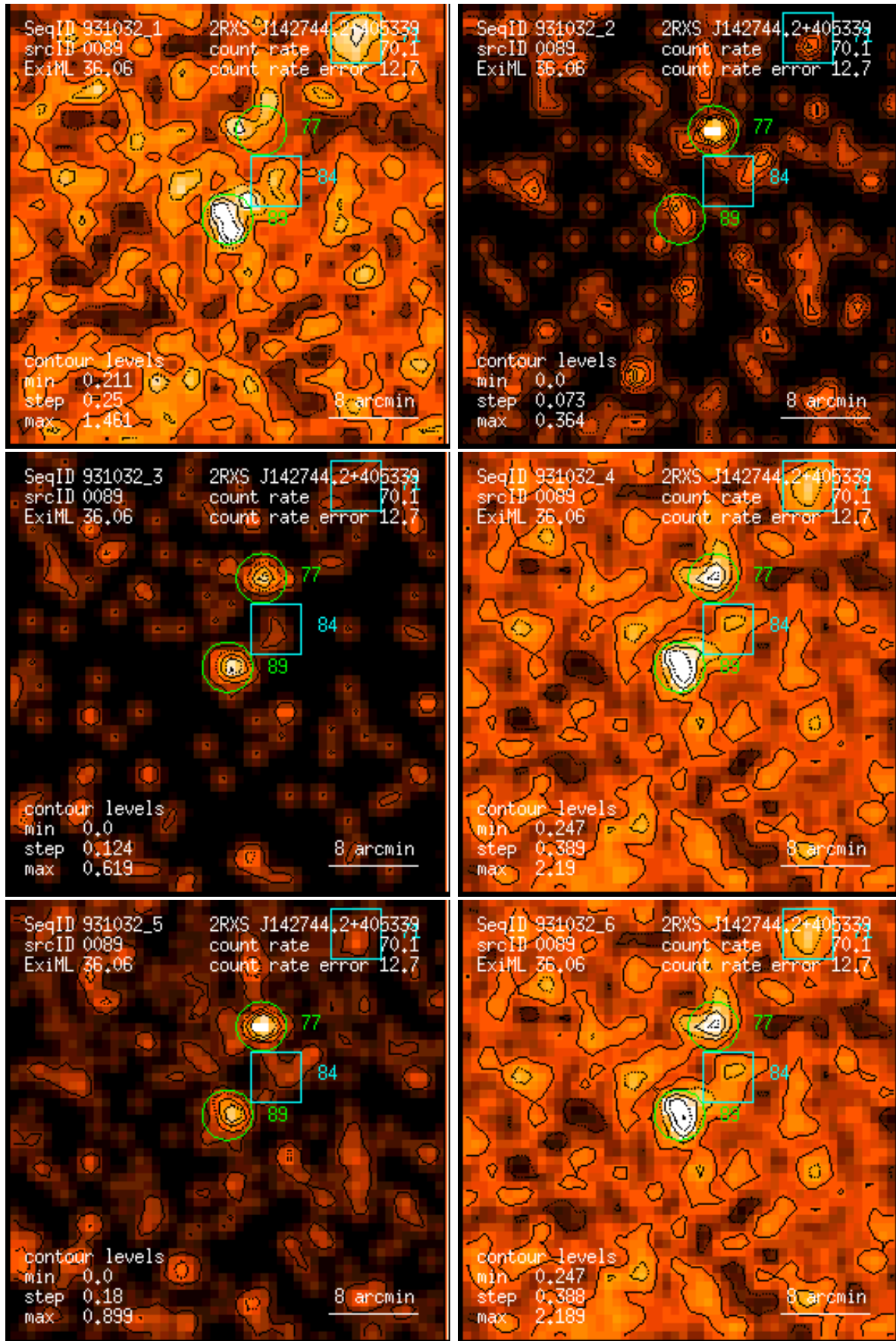
Figure 89: RASS 931032: detection 0089: band rate images, Gaussian filter: (1) PSPC channels 11 – 41, (2) 52 – 90, (3) 91 – 201, (4) 11 – 235, (5) 52 – 201, (6) 11 – 201. Broad band rates in counts/ks. Band rate contour levels in counts/ks/arcmin 2 .
