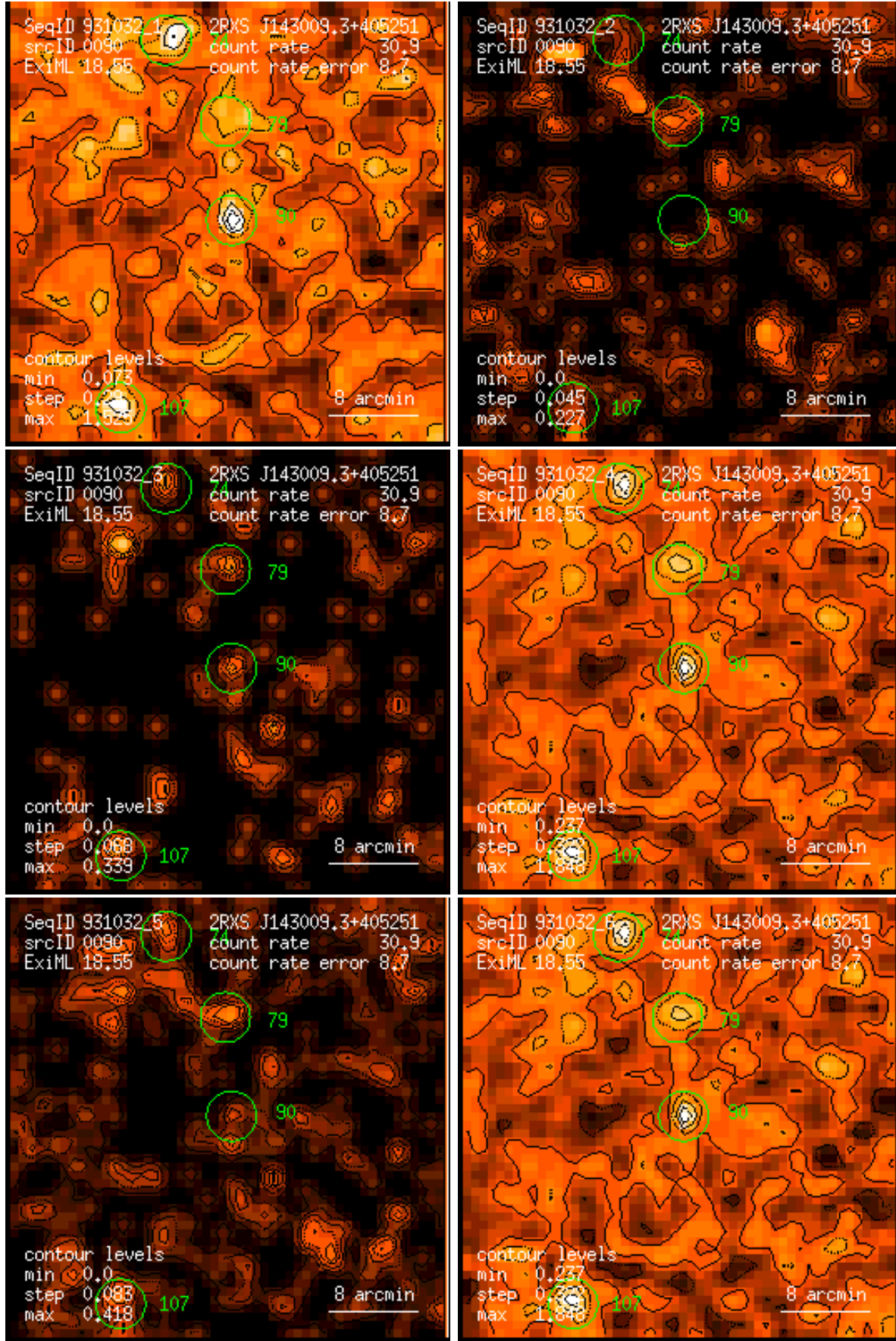
Figure 90: RASS 931032: detection 0090: band rate images, Gaussian filter: (1) PSPC channels 11 – 41, (2) 52 – 90, (3) 91 – 201, (4) 11 – 235, (5) 52 – 201, (6) 11 – 201. Broad band rates in counts/ks. Band rate contour levels in counts/ks/arcmin 2 .
