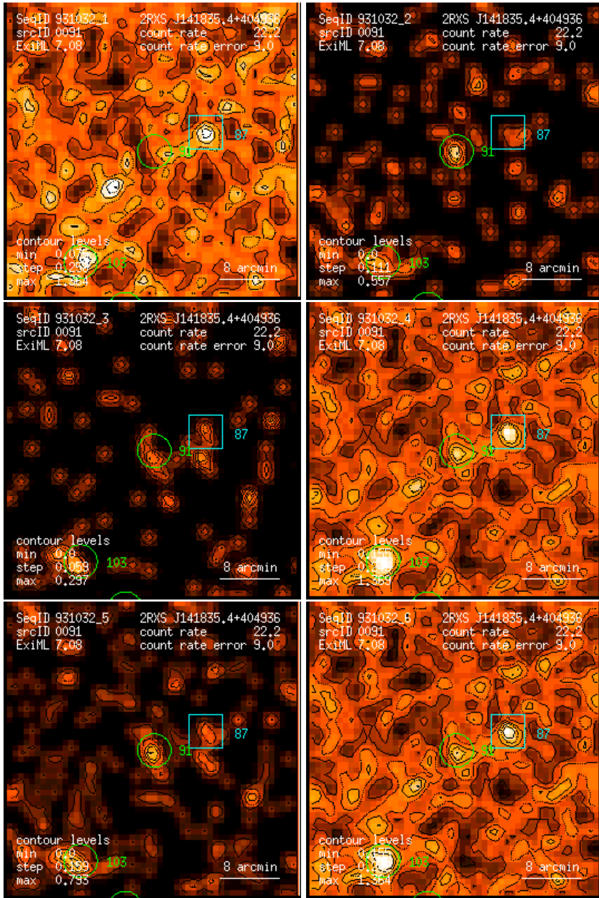
Figure 91: RASS 931032: detection 0091: band rate images, Gaussian filter: (1) PSPC channels 11 – 41, (2) 52 – 90, (3) 91 – 201, (4) 11 – 235, (5) 52 – 201, (6) 11 – 201. Broad band rates in counts/ks. Band rate contour levels in counts/ks/arcmin 2 .
