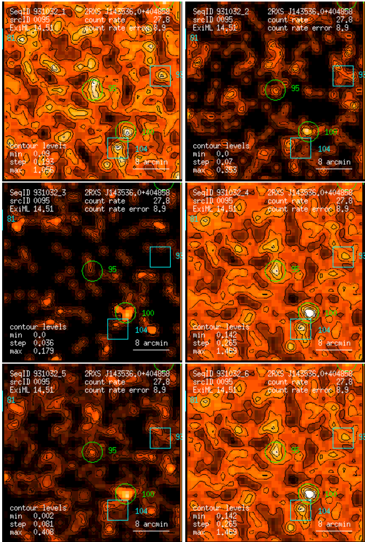
Figure 95: RASS 931032: detection 0095: band rate images, Gaussian filter: (1) PSPC channels 11 – 41, (2) 52 – 90, (3) 91 – 201, (4) 11 – 235, (5) 52 – 201, (6) 11 – 201. Broad band rates in counts/ks. Band rate contour levels in counts/ks/arcmin 2 .
