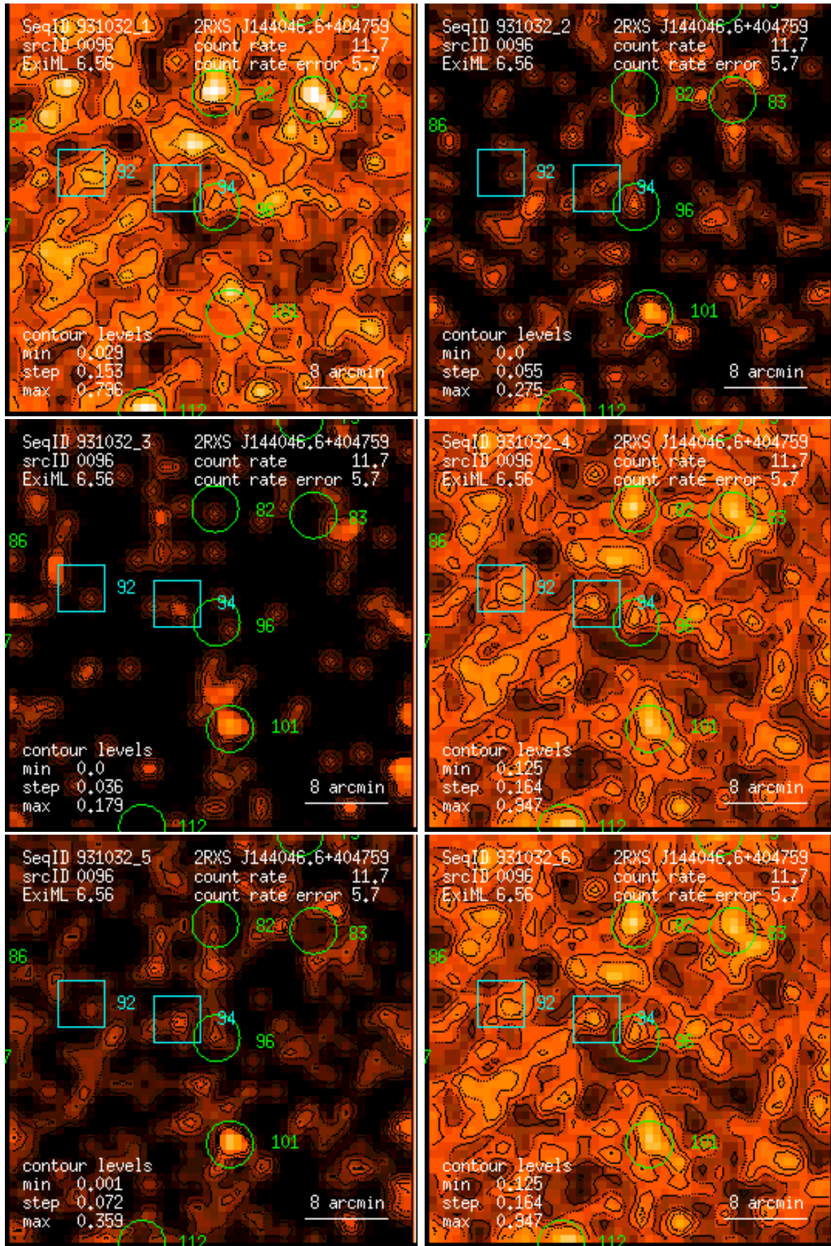
Figure 96: RASS 931032: detection 0096: band rate images, Gaussian filter: (1) PSPC channels 11 – 41, (2) 52 – 90, (3) 91 – 201, (4) 11 – 235, (5) 52 – 201, (6) 11 – 201. Broad band rates in counts/ks. Band rate contour levels in counts/ks/arcmin 2 .
