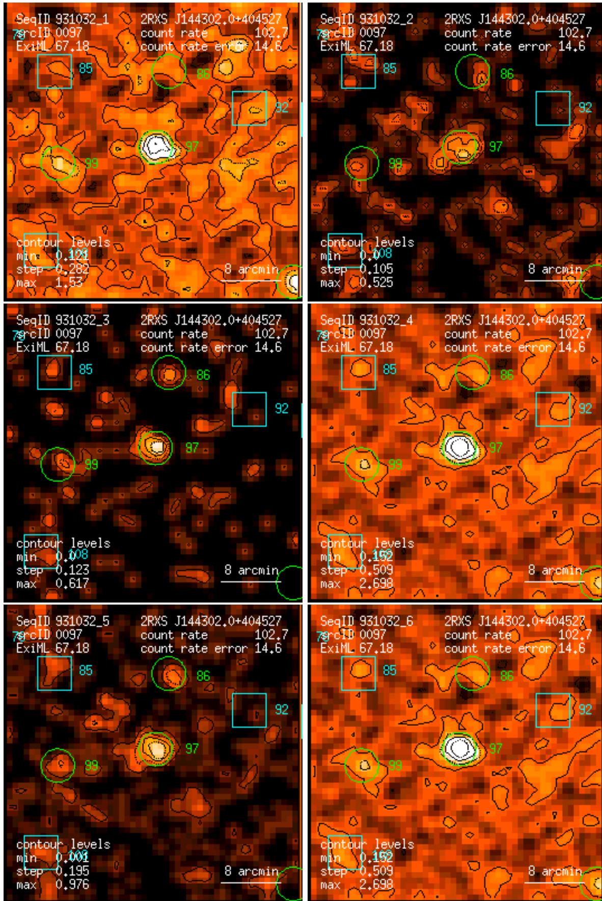
Figure 97: RASS 931032: detection 0097: band rate images, Gaussian filter: (1) PSPC channels 11 – 41, (2) 52 – 90, (3) 91 – 201, (4) 11 – 235, (5) 52 – 201, (6) 11 – 201. Broad band rates in counts/ks. Band rate contour levels in counts/ks/arcmin 2 .
